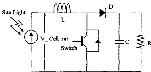
Fig. 2 Boost MPPT Block Diagram
