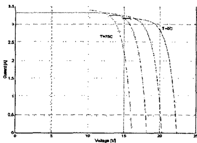
Fig. 3 V-I Characteristics Curves for Temperatures from 0. C to 75. C
