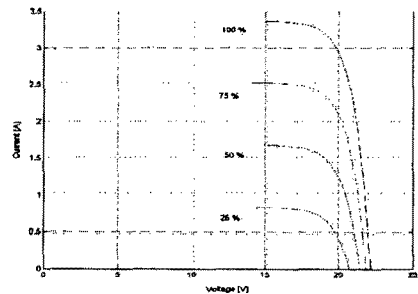
Fig. 5 V-I Characteristics Curves for Irradiance from 25% to 100%
