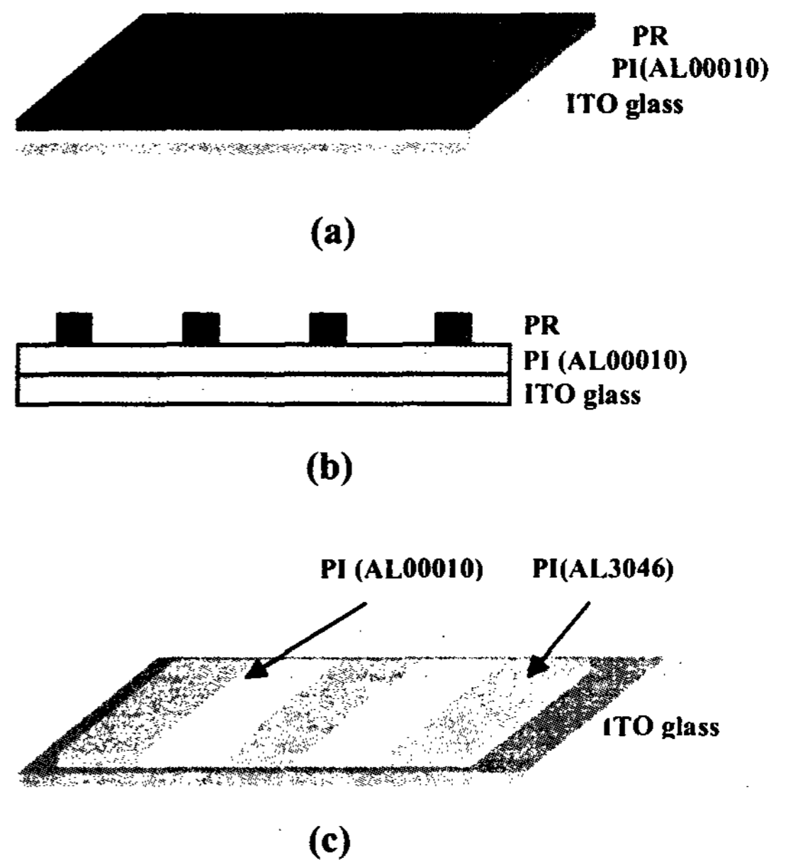
Fig. 4. The procedure to form multi domains: (a) PI (AL-00010) and PR coating on the ITO glass, (b) development after shedding the UV light, (c) removing PR after PI (AL-3046) coating.
