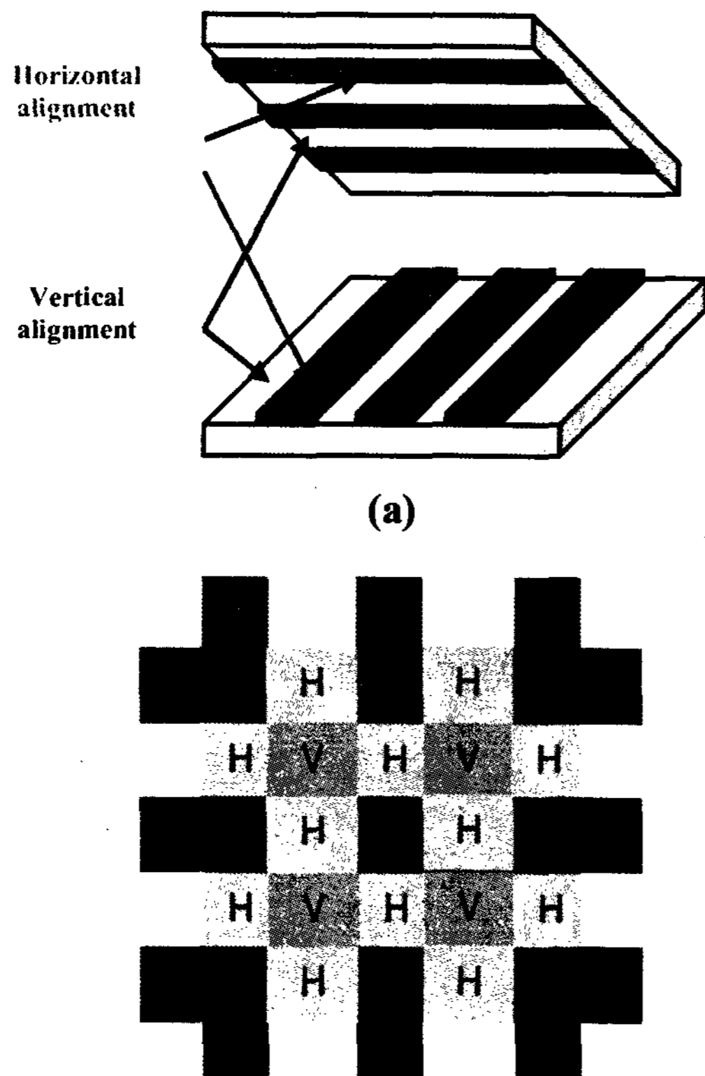
Fig. 3. Stripe patterns for multi domain: (a) stripe patterns on substrates, and (b) multi domain (S : splay, H : hybrid, V : vertical aligned).
