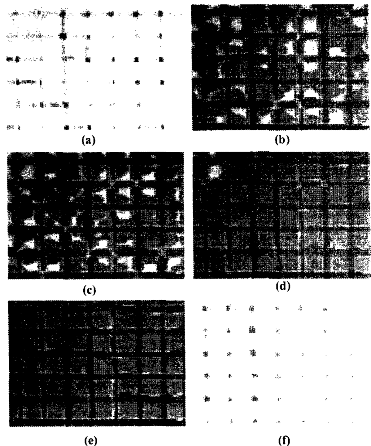
Fig. 6. Bend transition in each pixel with an applied voltage of 3 V: (a) without applied voltage, (b) 0.25 sec after 3 V is applied, (c) 0.5 sec later, (d) 1 sec later, (e) 2 sec later, and (f) an applied voltage of 2 V.
