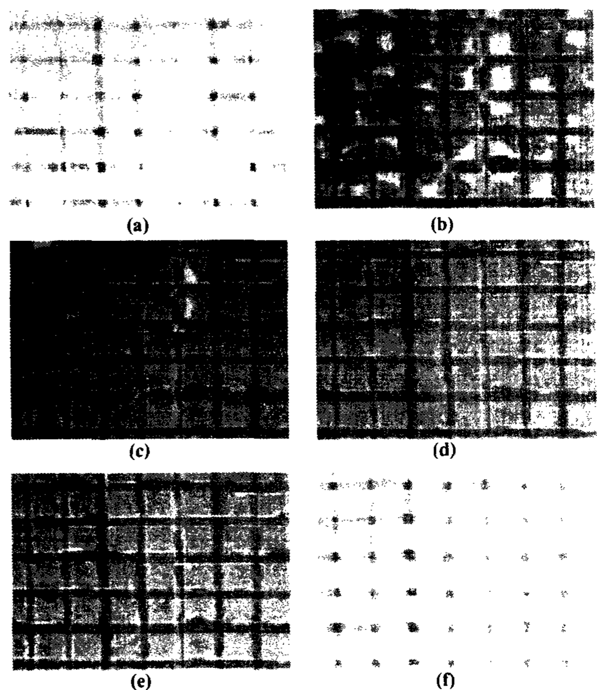
Fig. 7. Bend transition in each pixel with an applied voltage of 6 V: (a) Without applied voltage, (b) 0.25 sec after 6 V is applied, (c) 0.5 sec later, (d) 1 sec later, (e) 2 sec later, and (f) an applied voltage of 2 V.
