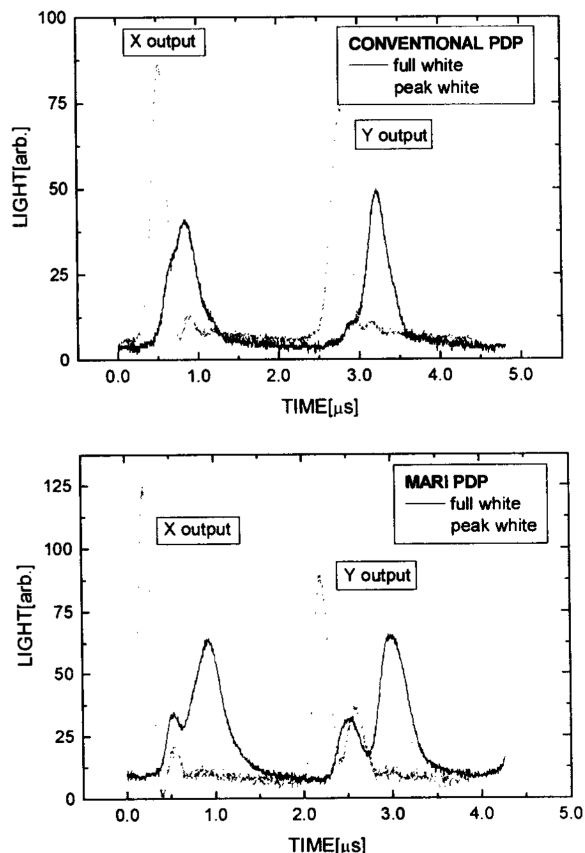
Figure 5 comparison of light intensity between conventional and MARI PDP
