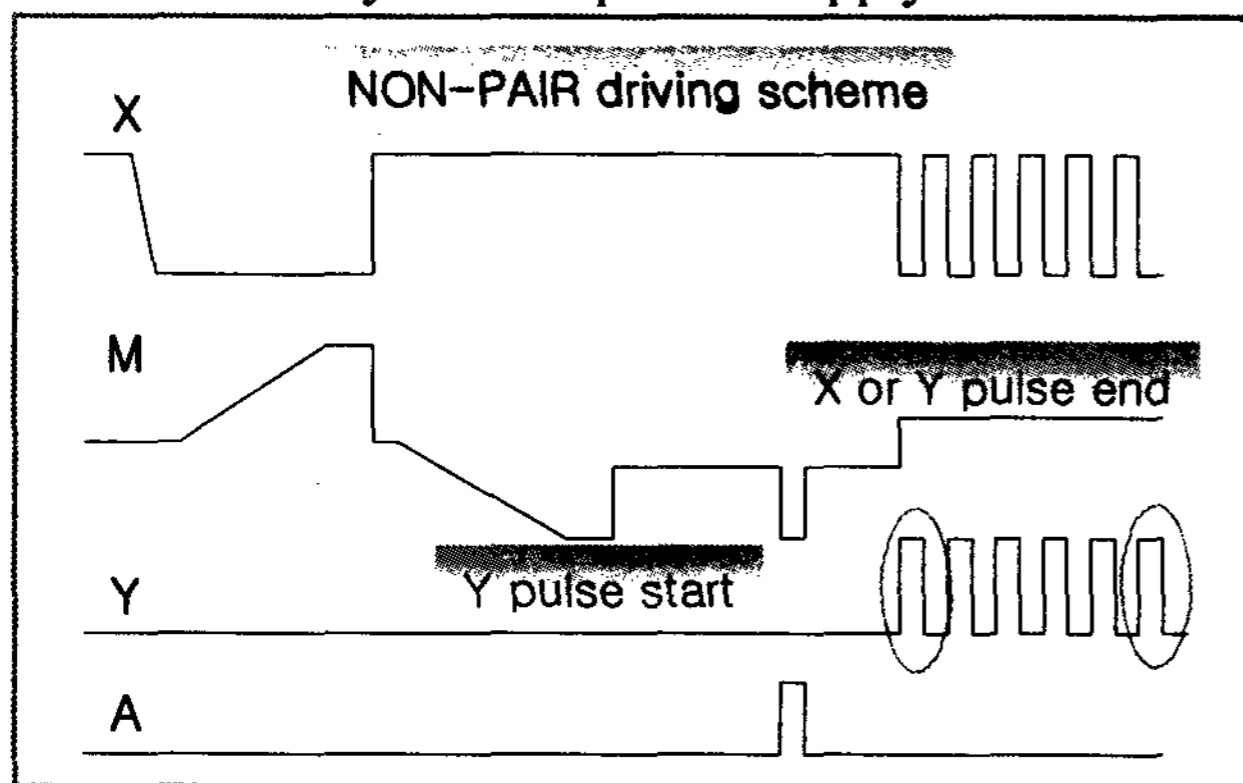
Figure 6 NON-PAIR driving scheme of MARI PDP.
