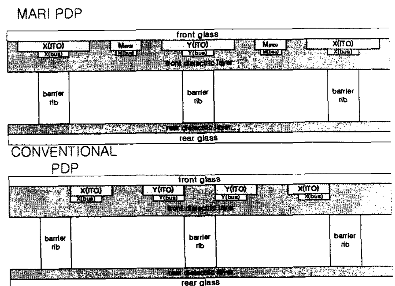
Figure 1 MARI PDP structure.
