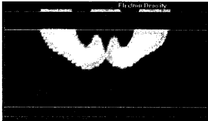
(b) X and Y electrode are common
