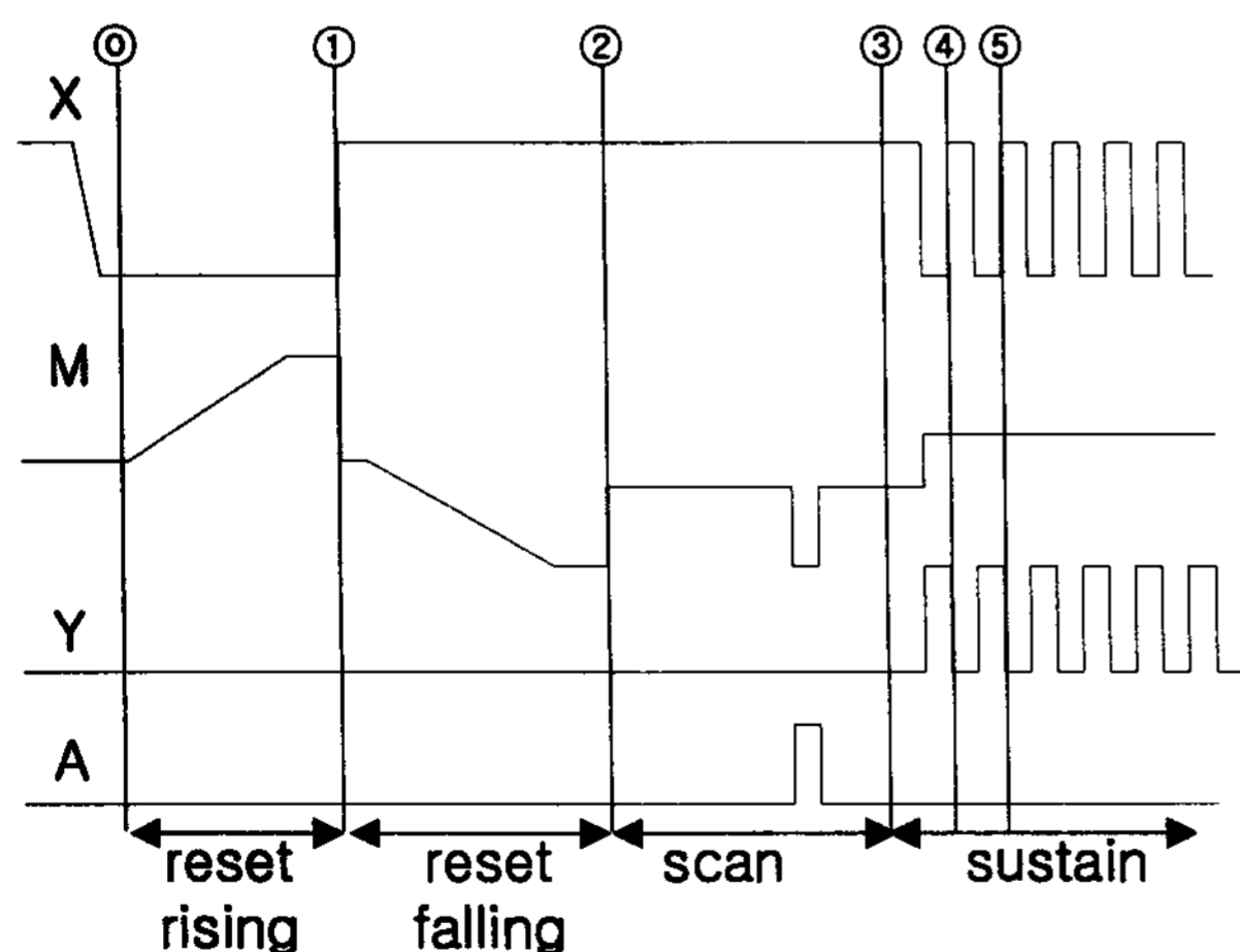
Figure 4 driving scheme of MARI PDP.
