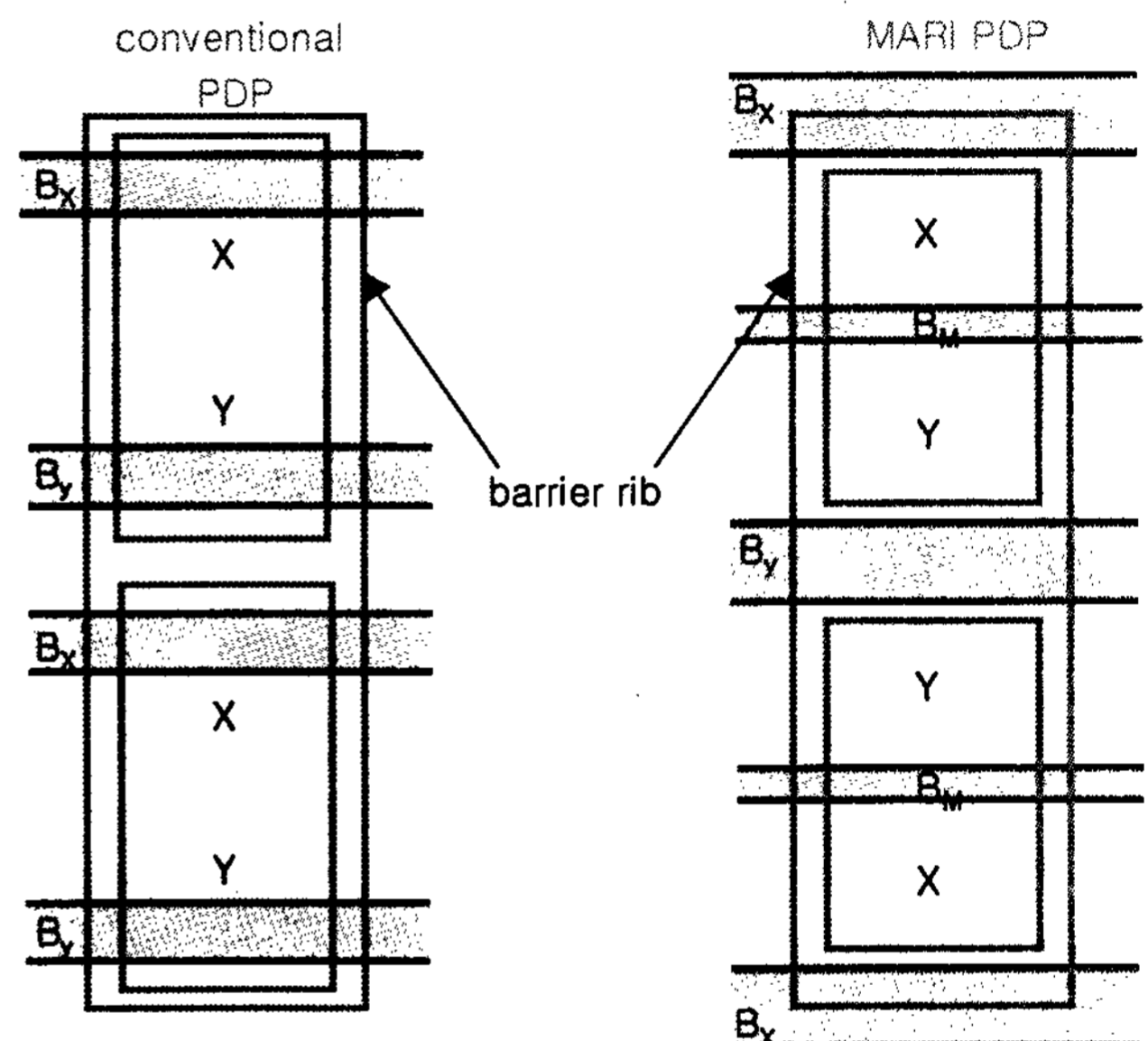
Figure 3 Electrode shape of MARI PDP
