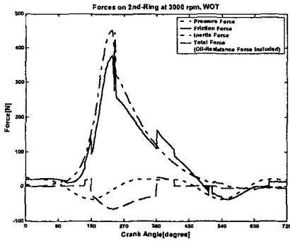
Fig. 8. Forces acting on second ring, 3000rpm WOT
