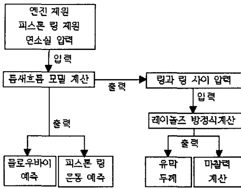
Fig. 5. Piston ring friction analysis procedure
