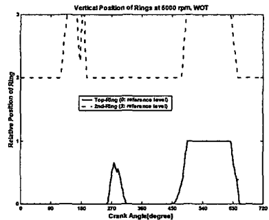
Fig. 13. Relative position of the ring, 5000rpm WOT. (First) Top ring, (Second) 2nd ring
