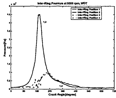
Fig. 10. Inter-ring pressure, 5000rpm WOT
