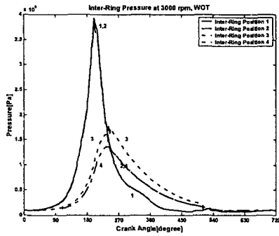
Fig. 6. Inter-ring pressure, 3000rpm WOT
