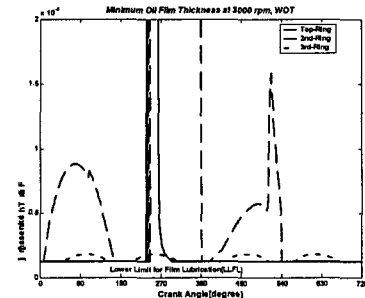
Fig. 14. Minimum oil film thickness, 3000rpm WOT
