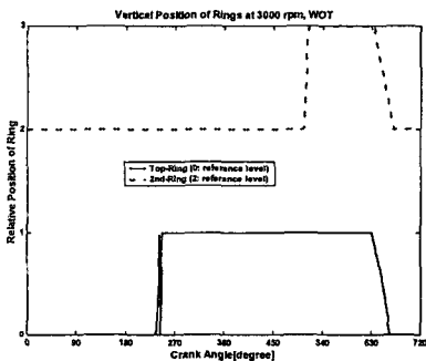
Fig. 9. Relative position of the ring, 3000rpm WOT. (First) Top ring, (Second) 2nd ring
