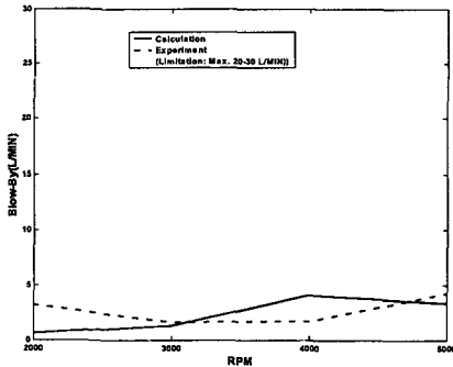
Fig. 18. Comparisons of the blowby between prediction and measurement at various speeds(WOT)
