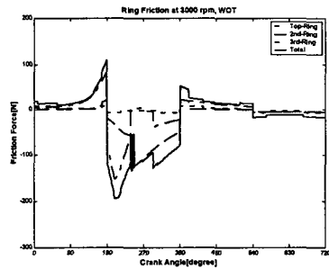
Fig. 16. Friction forces, 3000rpm WOT
