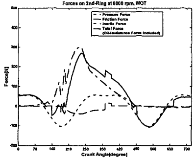
Fig. 12. Forces acting on second ring, 5000rpm WOT
