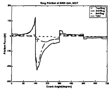
Fig. 17. Friction Forces, 5000rpm WOT
