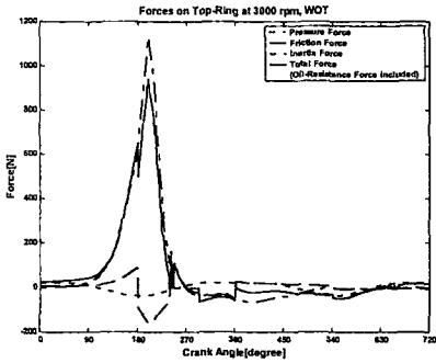
Fig. 7. Forces acting on top ring, 3000rpm WOT
