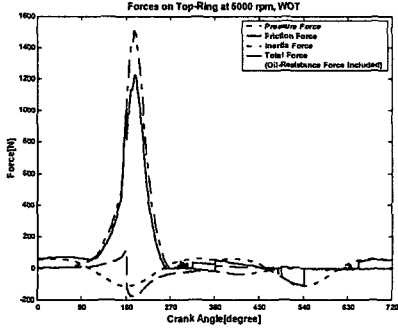
Fig. 11. Forces acting on top ring, 5000rpm WOT
