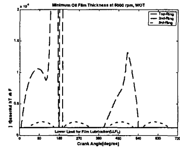
Fig. 15. Minimum oil film thickness, 5000rpm WOT
