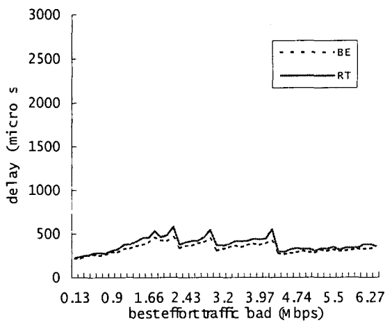
Fig. 12. The delay with congestion control when the real time bandwidth requirement is 3.027 Mbps
