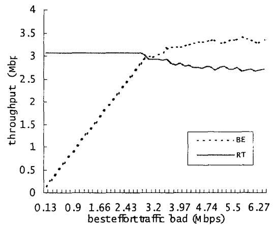
Fig. 9. The throughput with no congestion control when the real time bandwidth requirement is 3.027 Mbps
