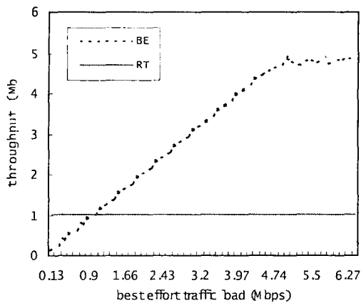
Fig. 7. The throughput when the real time bandwidth requirement is 1 Mbps
