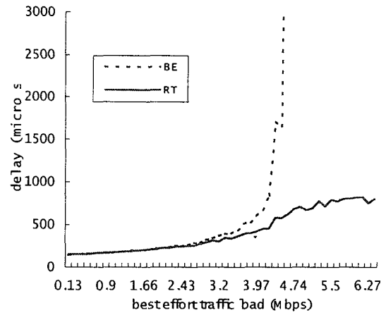
Fig. 8. The delay when the real time bandwidth requirement is 1 Mbps
