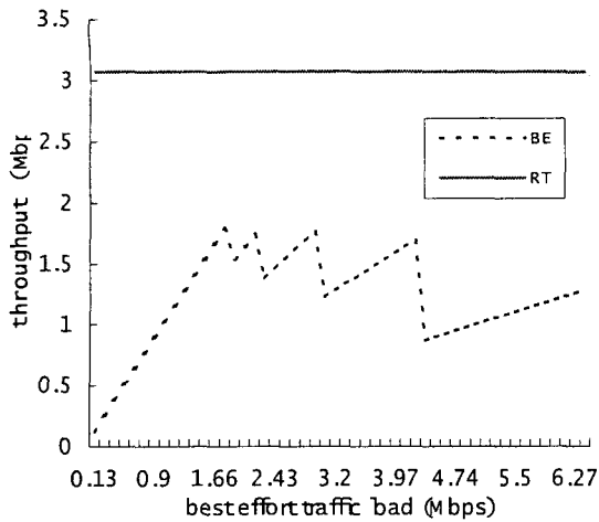
Fig. 11. The throughput with congestion control when the real time bandwidth requirement is 3.027 Mbps
