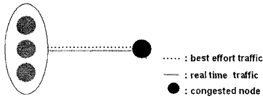
Fig. 5. Network model
