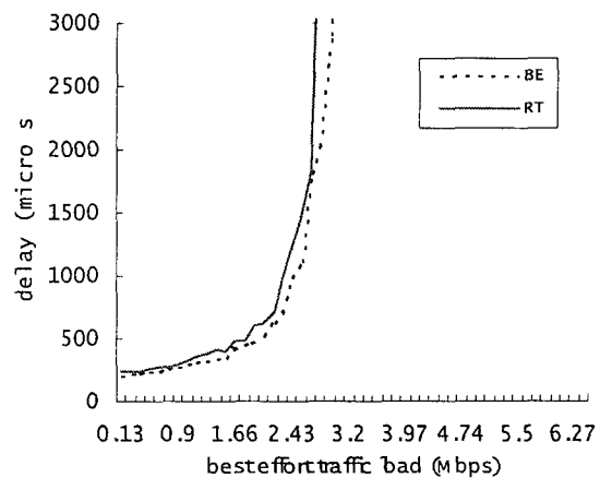
Fig. 10. The delay with no congestion control when the real time bandwidth requirement is 3.027 Mbps
