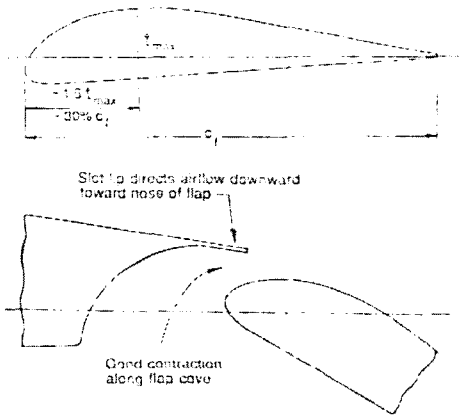
Fig. 6 Design guideline of slotted flap
