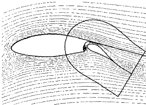
Fig. 11 Streamline (Flap#2, \delta_f=30^\circ , \alpha=8^\circ )
