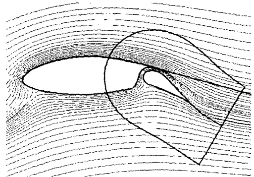
Fig. 13 Streamline (Flap#9, \delta_f=30^\circ , \alpha=8^\circ )
