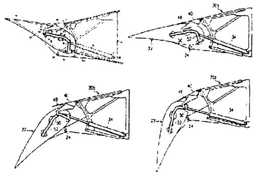
Fig. 7 Concept of Tiltrotor Flaperon
