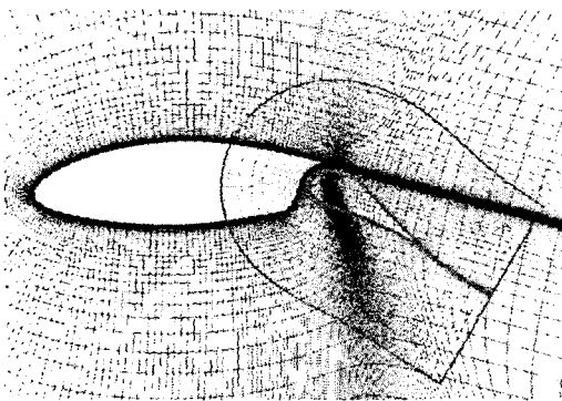
Fig. 8 Grid around airfoil and flap
