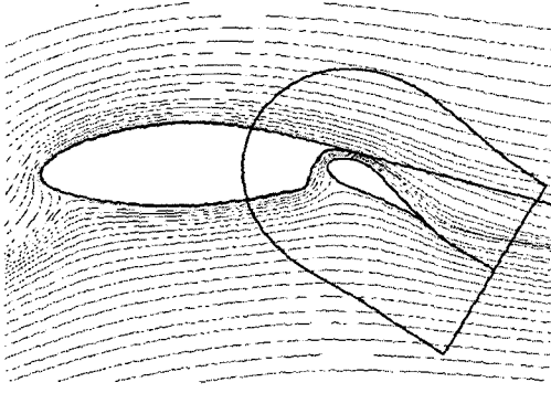
Fig. 12 Streamline (Flap#6, \delta_f=30^\circ , \alpha=8^\circ )
