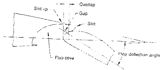
Fig. 5 Geometrical definition of slotted flap
