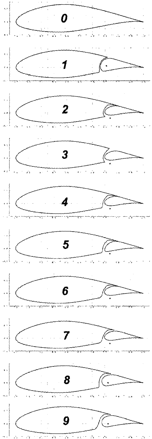
Fig. 9 Flaperon candidates
