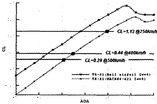
Fig. 2 Lift curve of SUAV(TR-S1)
