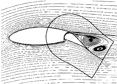
Fig. 10 Streamline (Flap#1, \delta_f=30^\circ , \alpha=8^\circ )
