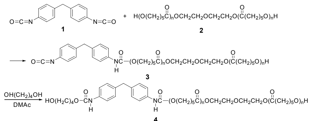
Scheme 1. The Synthetic route of Shape memory polymer
