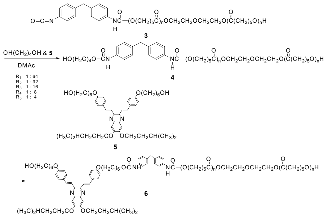
Scheme 2. The Synthetic route of Multi-functional Shape memory polymer
