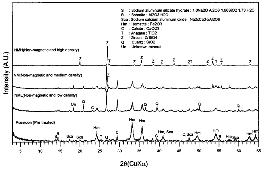
Fig. 3. XRD patterns of pre-activated samples. NML, NM and NMH are samples separated by magnetic separator and shaking table.
