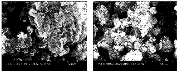
Fig. 4. SEM images of pre-treated and post-treated samples.
