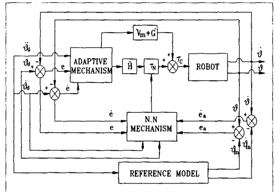
Fig. 5 The block diagram of adaptive-neuro controller.
