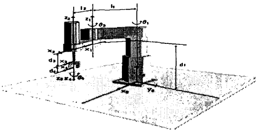
Fig. 3 Coordinates frame of SCARA robot.
