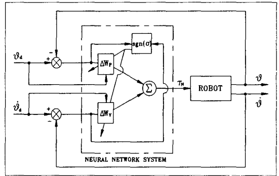
Fig. 4 The block diagram of neural network.
