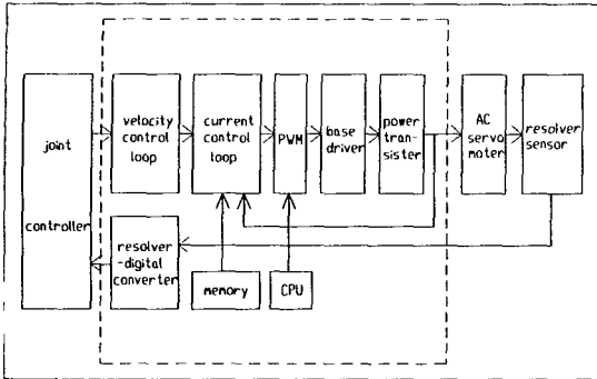
Fig. 6 AC joint driver.
