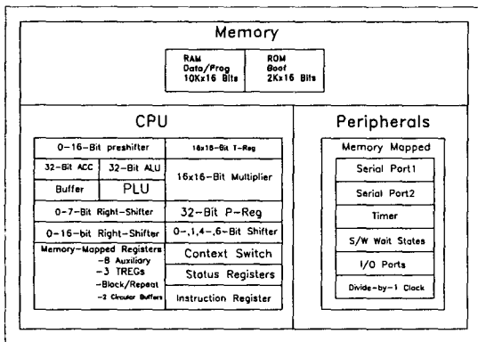
Fig. 7 TMS320C50 block diagram.
