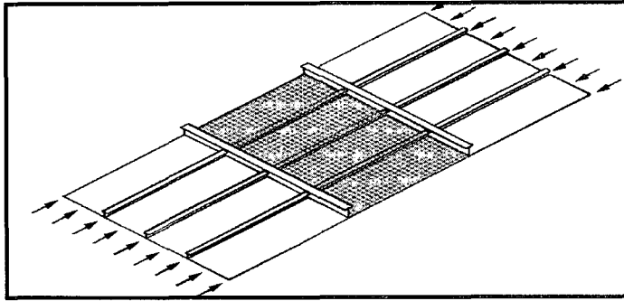
Fig. 6 FEA model - One bay SPM (Stiffener Panel Combination)
