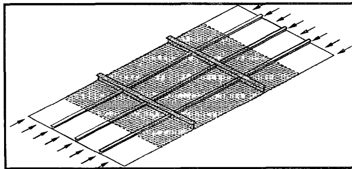
Fig. 7 FEA model - Two bay SPM (Stiffener Panel Combination)
