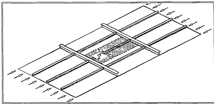
Fig. 4 Theoretical model - One bay PSC (Plate-Stiffener Combination with b_e=b )
