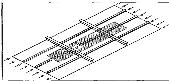
Fig. 5 FEA model - Two bay PSC (Plate-Stiffener Combination)
