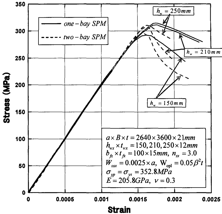
Fig. 9 A comparison stress with strain curves of the stiffened plate under axial compression according to the web height and analysis range
