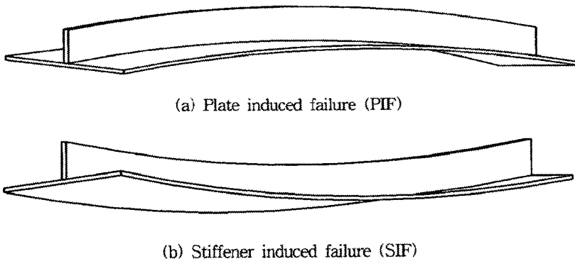
Fig. 2 Collapse modes of a plate induced combination
