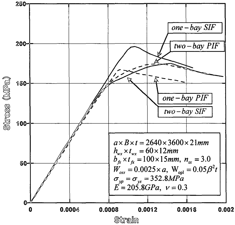
Fig. 8 A comparison stress with strain curves of the stiffened plate under axial compression according to the analysis range
