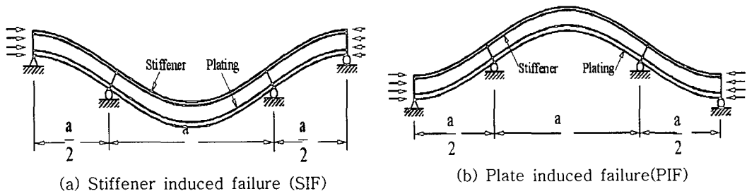
Fig. 3 A Schematic representation of PIF failure and SIF patterns in the two bay model
