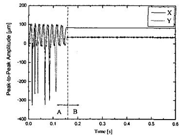
Fig. 11 Signal of a seal rotation
