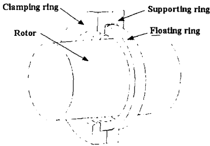
Fig. 2 Construction of floating ring seal
