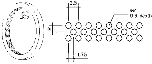
Fig. 4 Damper floating ring seal
