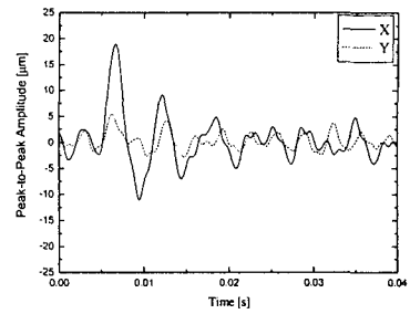
(a) Displacement signal between housing and shaft
