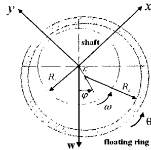
Fig. 7 Coordinate of floating ring seal
