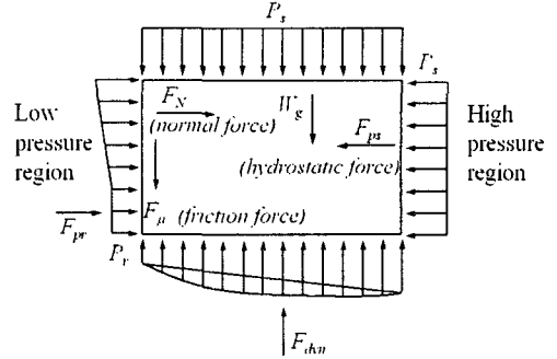
Fig. 3 FBD of floating ring seal
