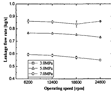
(b) Damper floating ring seal
