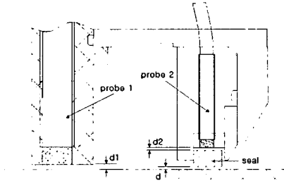
Fig. 5 Measuring the lock-up position
