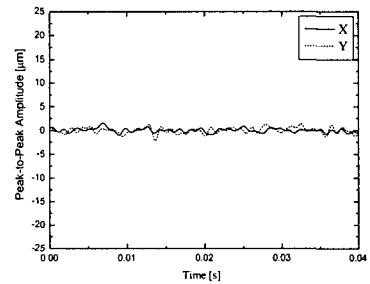
(b) Displacement signal between housing and seal
