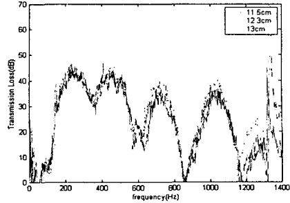
Fig. 16 Comparison of transmission loss for 3 cases
