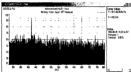
Fig. 2 FFT Measurement for noise (93.5dB/416.5Hz)
