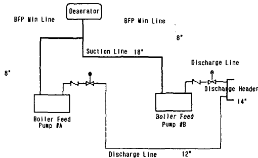
Fig. 1 Schematic of flow through the BFP
