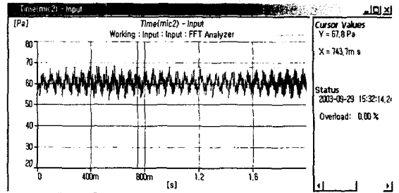
Fig. 3 Time chart
