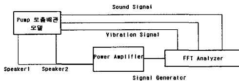
Fig. 9. System configuration
