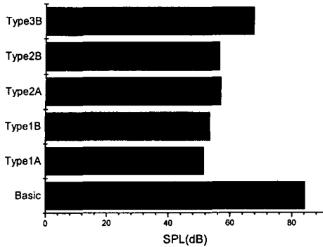
Fig. 14 SPL for each type
