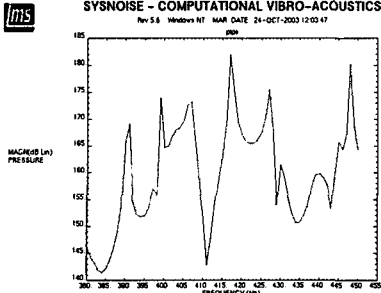
Fig. 7 Sound Pressure at Field Point 186
