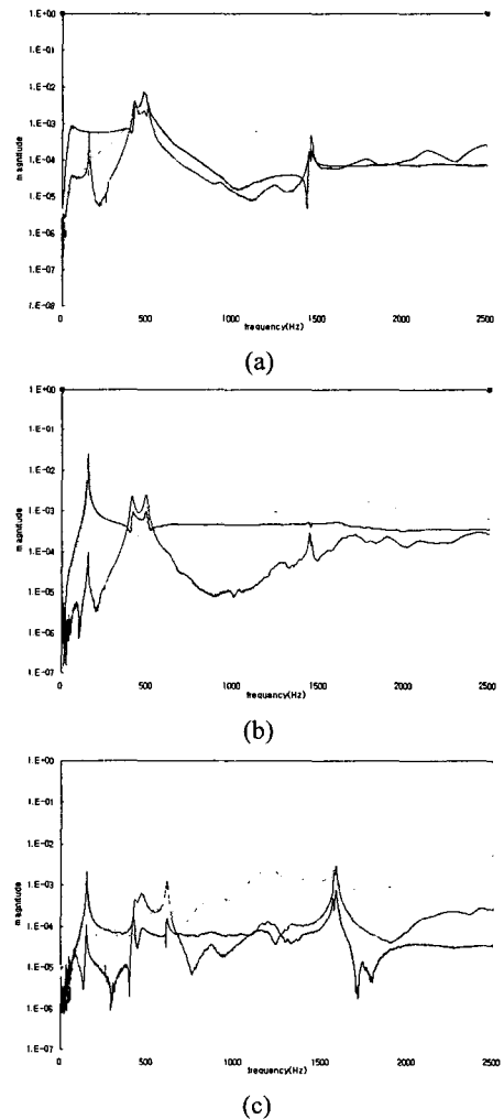
Fig. 2 Frequency response curve at (a) axial excitation, (b) lateral excitation and (c) vertical excitation.
