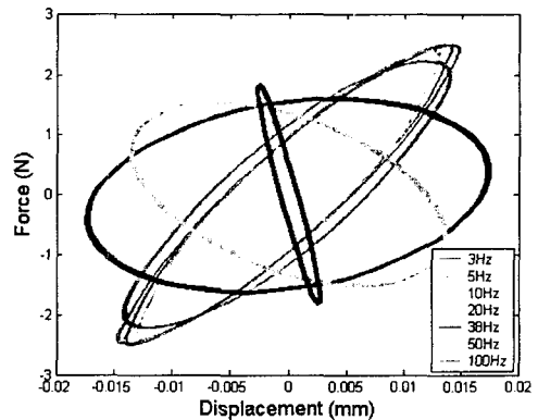
Fig. 5 Force-displacement relation at various excitation frequencies
