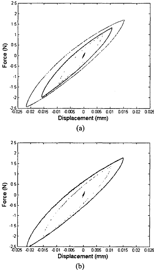
Fig. 4 Hysteresis curves for the force-displacement relation for (a) 0.5Hz and (b) 1.0Hz.
