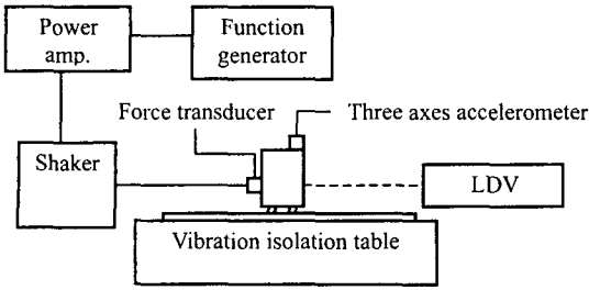
Fig. 1 Experimental setup for the LM guide vibration test
