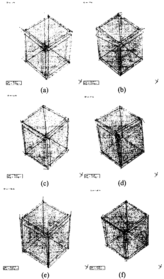
Fig. 3 Mode shapes. (a) translational, (b) rolling, (c) yawing, (d) pitching, (e) bouncing and (f) high-order rolling.
