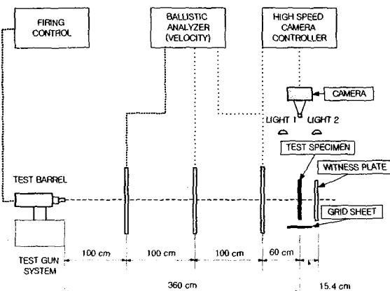
Fig. 1 Schematics of the ballistic range setup for hi Fig. 2 fiber composites materials after high velocity impact test
