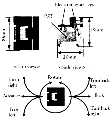
Fig. 10 Principle of microscopic locomotion of micro robot
