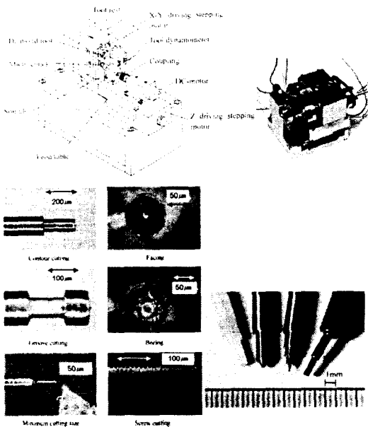
Fig. 4 Micro lathe and shape cutting
