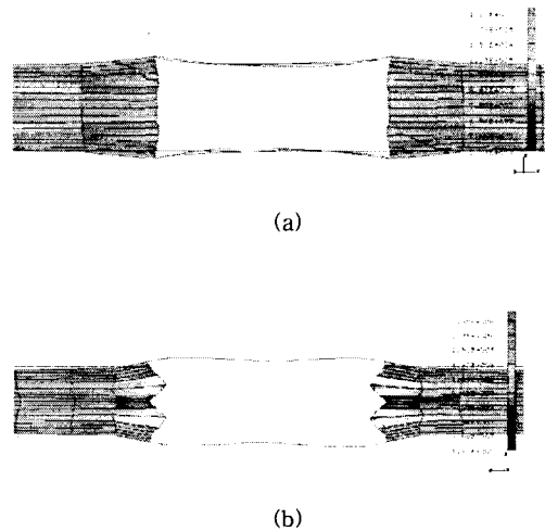
Fig. 2 Optimized shape of [ \pm 45/0/90 ] s plate loaded in biaxial and shear stress.
