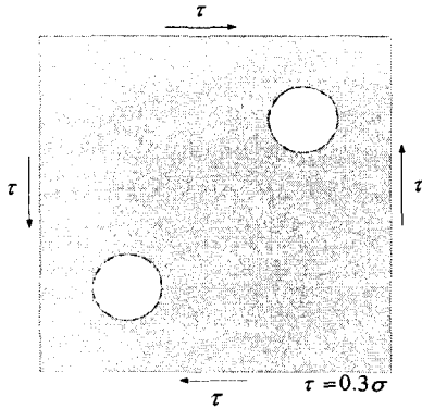
Fig. 6 [\pm 45/0/90] , Plate loaded in shear stress.
