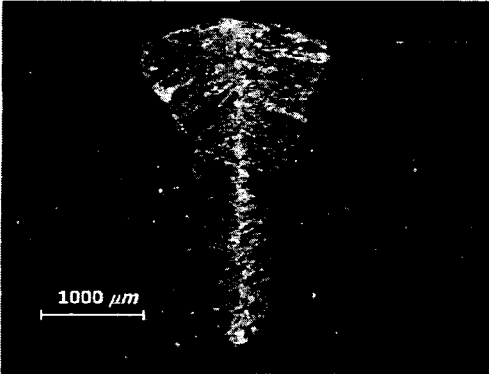
Fig. 3 Cross-sectional area of bead on plate welding at P=1.4kW, v=1.0m/min and z=0.5mm
