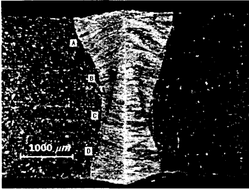
Fig. 7 Butt welding Cross-sectional area of the laser beam power at P=1.6kW , v=1.0m/min and z=0.5mm
