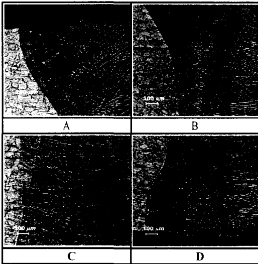
Fig. 8 Photographs showing laser butt welding ( P=1.6kW , v=1.0m/min , z=0.5mm )
