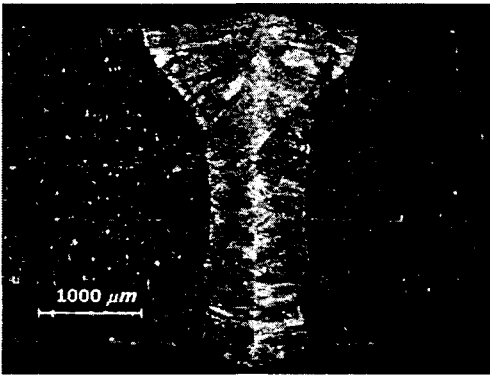
Fig. 4 Cross-sectional area of bead on plate welding at P=1.5kW, v=1.0m/min and z=0.5mm
