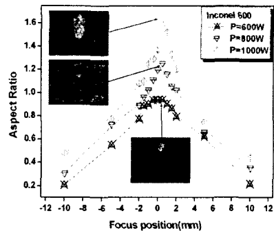
Fig. 2 Relation between position of focus and aspect ratio
