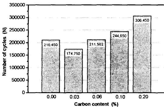
Fig. 8 Relation between fatigue life and carbon content
