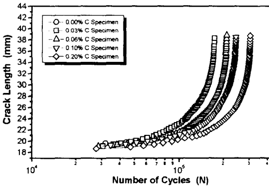
Fig. 7 Relation between crack length and number of cycles
