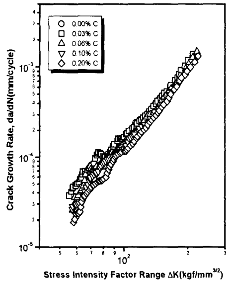
Fig.9 Relation between crack propagation rate and stress intensity factor range
