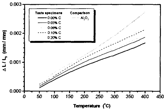
Fig. 4 Relation between thermal expansion and temperature
