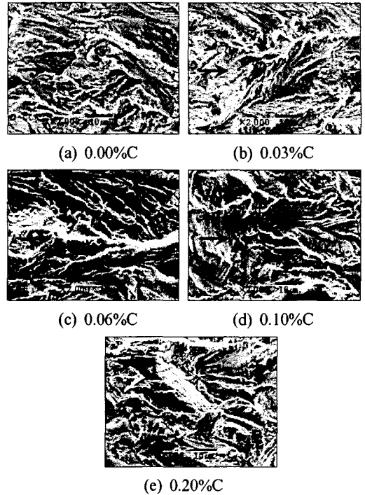
Photo. 1 SEM fractographs of the fatigue test specimens( \times 2000 )
