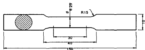
Fig. 1 Geometry of the tensile and compressive test specimen
