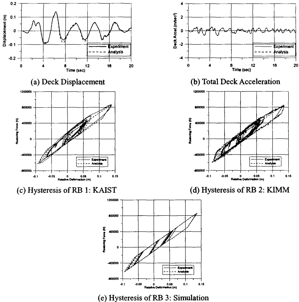
Fig. 9 Results of On-line Network Testings
