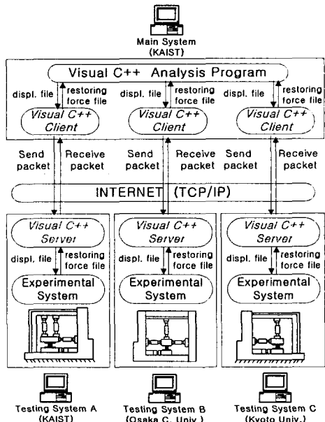
Figure 3 Configuration II (Using TCP/IP)
