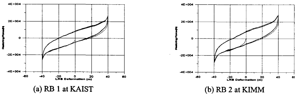
Fig. 8 Hysteresses for Cyclic Tests on RB Specimens
