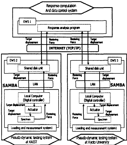
Figure 2 Configuration I (Using TCP/IP and SAMBA)
