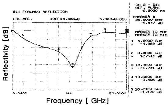
(c) Reflection coefficient of mixed MnZn ferrite absorber with natural lacquer.
