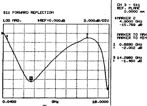
(d) Electromagnetic absorber's reflection coefficient that thickness is 4 mm
