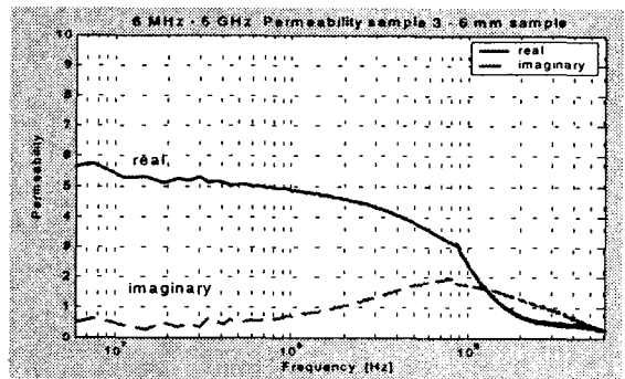
(b) Complex permeability of MnZn ferrite absorber mixed with silicone rubber.
