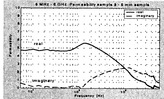
(a) Complex permeability of MnZn ferrite absorber mixed with CPE.
