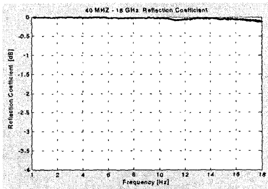
(a) Purity CPE's reflection coefficient that thickness is 5 mm.
