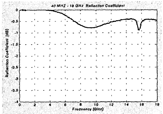
(c) Purity Natural Lacquer's reflection coefficient that thickness is 5 mm.
