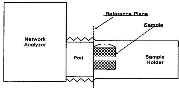
Fig. 1 Reflection coefficient measurement system of sample.
