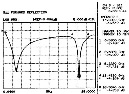
(f) Electromagnetic absorber's reflection coefficient that thickness is 6 mm
