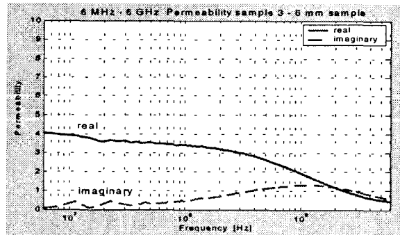
(c) Complex permeability of MnZn ferrite absorber mixed with natural lacquer.
