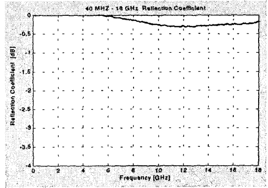
(b) Purity Silicone's reflection coefficient that thickness is 5 mm.
