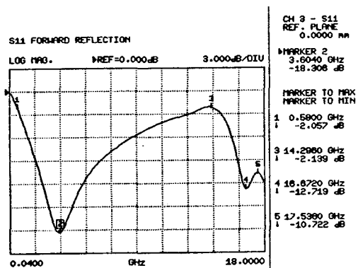
(e) Electromagnetic absorber's reflection coefficient that thickness is 5 mm
