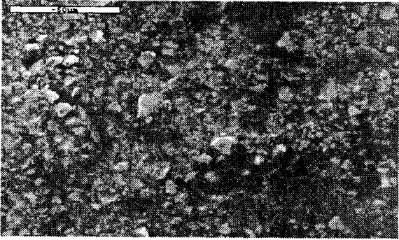
(b) MnZn ferrite mixed with silicone rubber.
