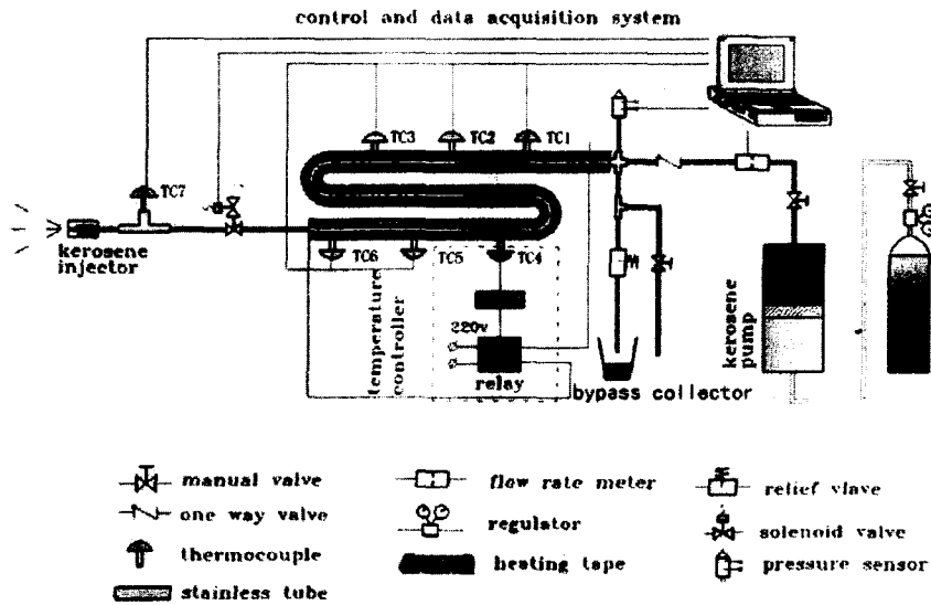
Figure 2 Schematic of kerosene delivery and heating system.
