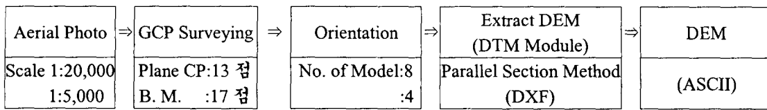
Fig. 9. Process for DEM Production by Analytical Plotter
