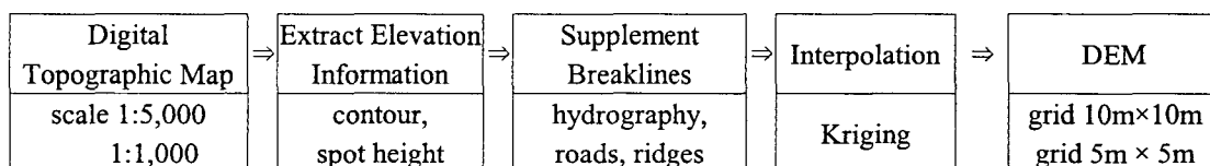
Fig. 8. Process for DEM Production from Digital Topographic Map
