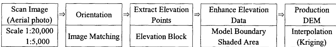
Fig. 10. Process for DEM Production by Digital Plotter
