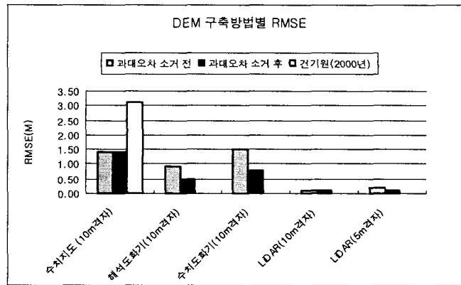
Fig. 11. RMSE related to DEM Production Method (grid 10m)
