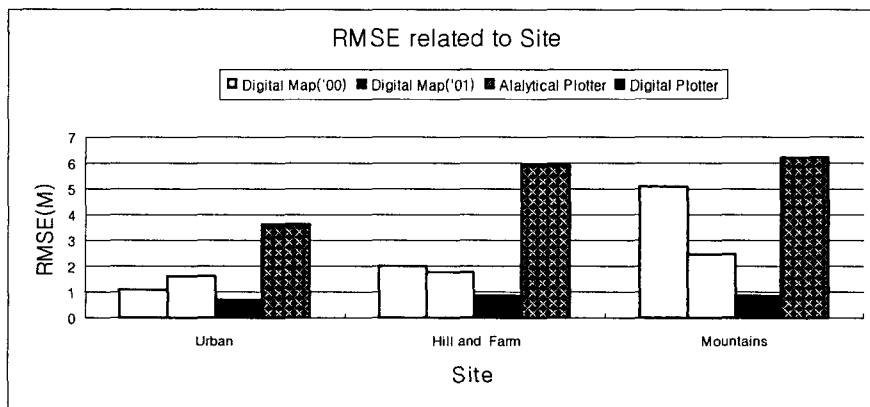
Fig. 12. RMSE related to Site(Grid 10m)
