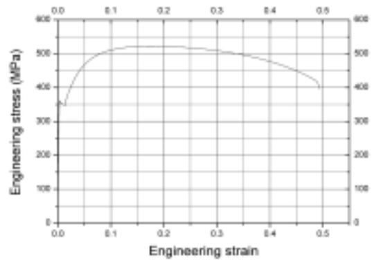
Fig. 4 Tensile strain-stress curve
