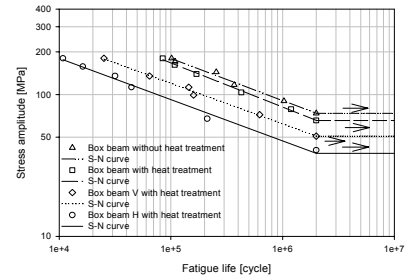
Fig. 22 S-N curve of the box beam specimens
