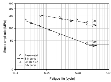
Fig. 15 BM and CN
