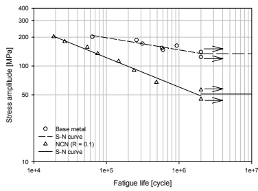
Fig. 14 BM and NCN
