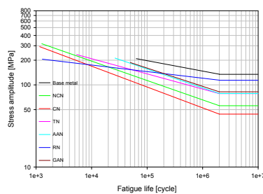
Fig. 21 S-N curves for the various welded joints
