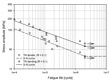
Fig. 20 TN tensile and TN bending
