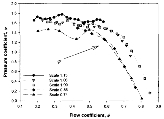
(b) 1000 rpm
