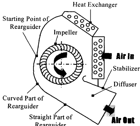
Fig. 1 Schematic of a cross-flow fan.
