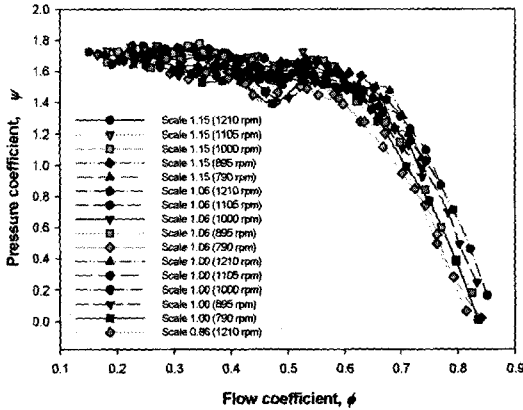
Fig. 6 Pressure coefficients with various Reynolds numbers.
