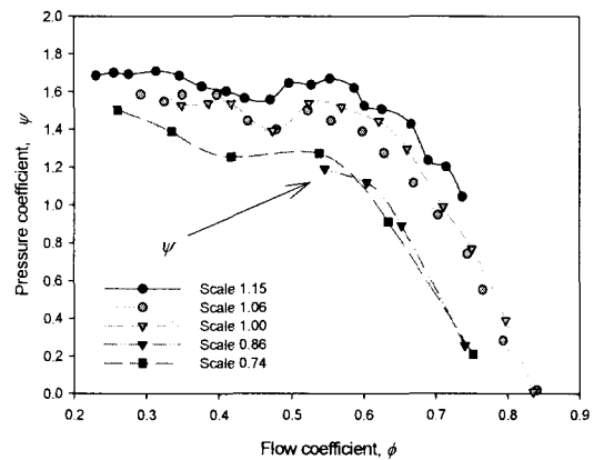
(c) 790 rpm
