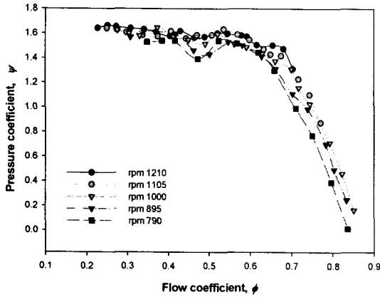
Fig. 4 Pressure coefficients with various rpms for scale=1.00.
