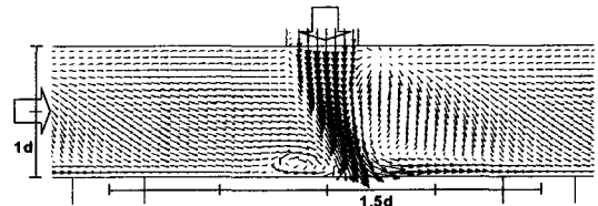
(a) On injection plane ( z/d=3.0 )
