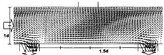
(b) On effusion plane ( z/d=0.0 )
