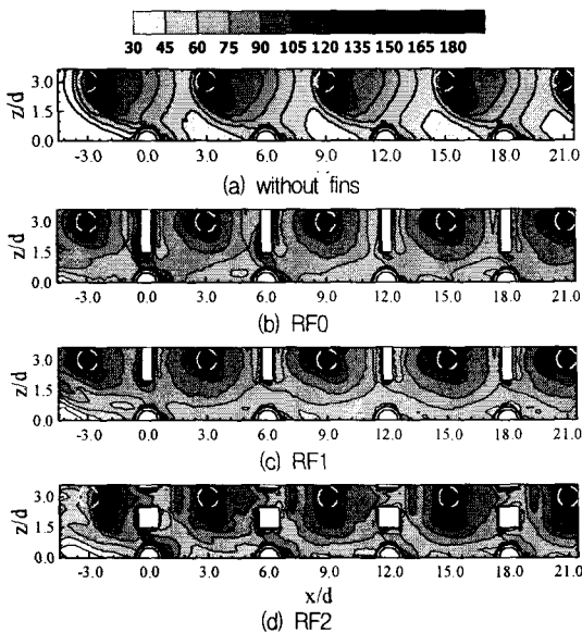
Fig. 5 Contour plots of Sh impingement/effusion cooling with rectangular fins at M=1.0
