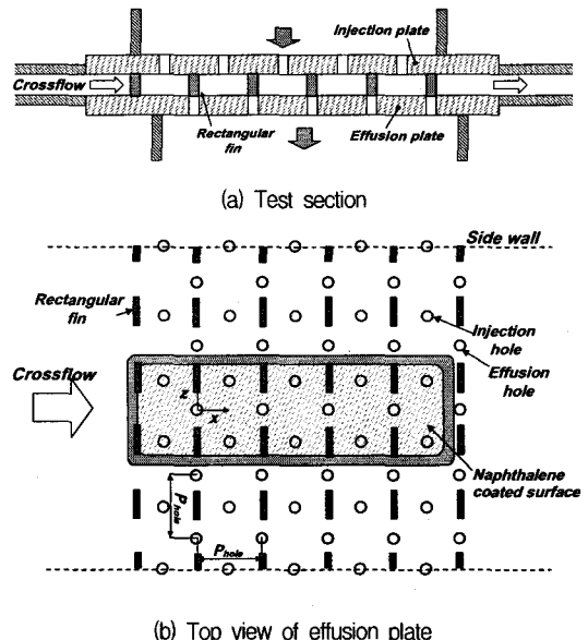
Fig. 1 Schematic view of test section
