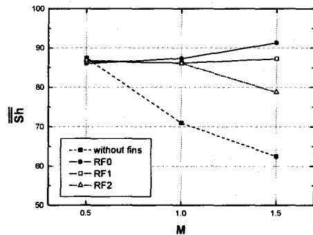
Fig. 8 Overall average Sh for impingement/effusion cooling at various blowing ratios
