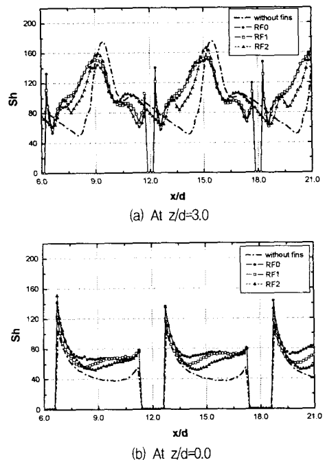
Fig. 6 Local distributions of Sh for impingement/effusion cooling with various fin configurations at M=1.0
