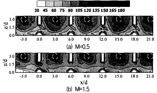
Fig. 7 Contour plots of Sh for RF1 case at different blowing ratio
