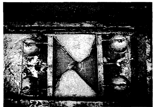
Fig.11 Floating skimmer installed in the water bath of actual paint booth
