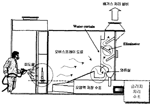
Fig. 1 Schematic of wet-type paint booth
