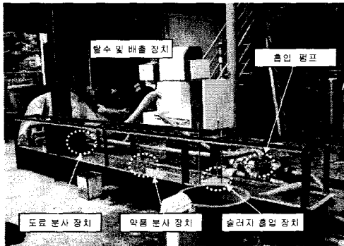
Fig. 4 Experimental setup for the sludge treatment system with floating skimmer
