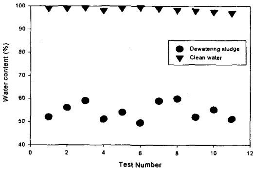
Fig. 13 Water contents of waste water and sludge treated by the present system( Company A )
