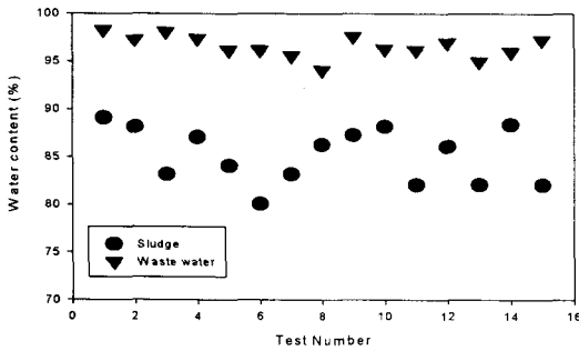
Fig. 16 Water contents of waste water and sludge treated by human operation( Company B )
