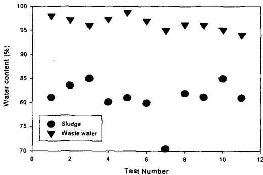
Fig. 12 Water contents of waste water and sludge treated by human operation( Company A )
