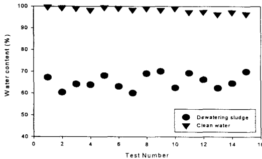
Fig. 17 Water contents of waste water and sludge treated by the present system( Company B )
