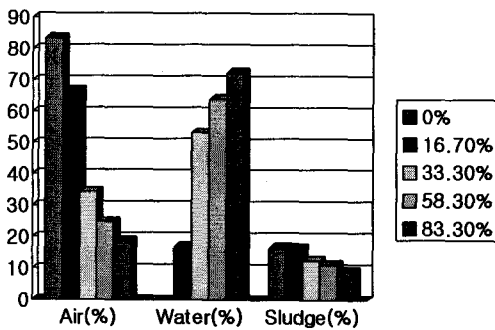
Fig. 8 Suction flow comparisons of air, water and sludge
