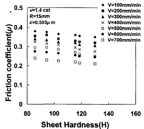
Fig. 2 Friction coefficients associated with sheet surface hardness in various punch speed.
