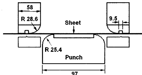
Fig. 3 Tooling geometry of 2-D stretching process.
