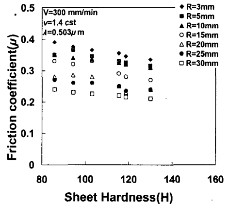
Fig. 1 Friction coefficients associated with sheet surface hardness in various punch corner radii.
