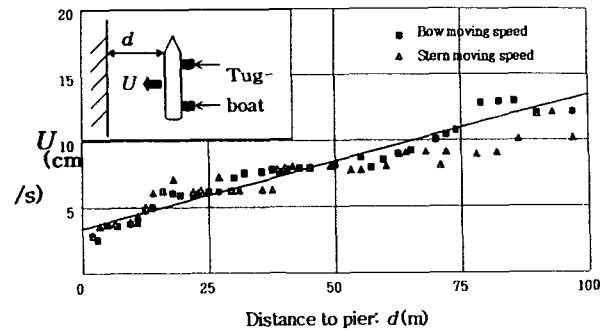
Fig. 1 Lateral berthing speed with the distance to pier
