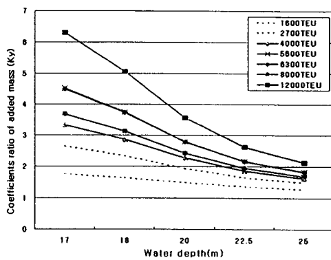
Fig.5 Coefficient ratio of sway added mass
