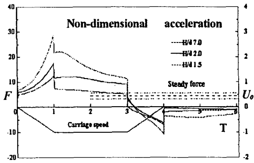
Fig. 2 Hydrodynamic forces under the lateral motion
