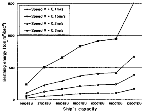
Fig.3 Berthing energy with the ship's capacity
