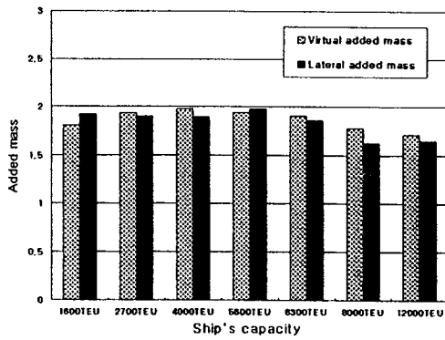
Fig. 4 Comparison of added mass
