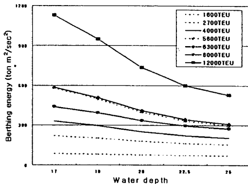
Fig.6 Berthing energy with the water depth (V=1.5cm/s)
