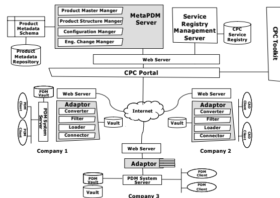
Fig.3 System Architecture
