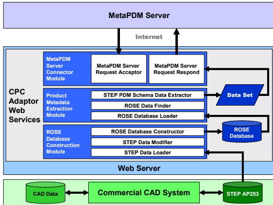
Fig.6 CPC Adaptor system architecture
