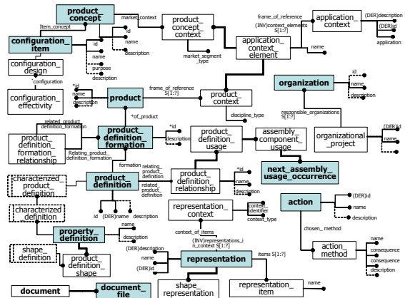
Fig.5 Product Data in ISO STEP PDM Schema
