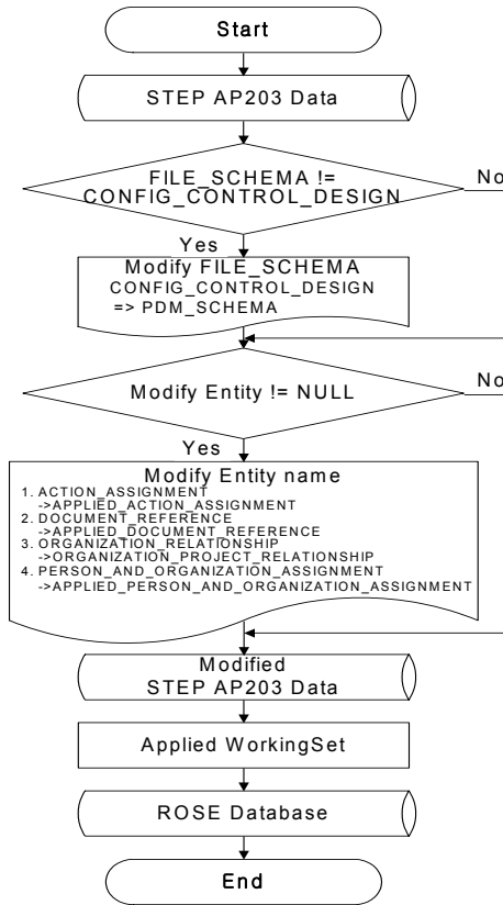
Fig.8 ROSE database construction module
