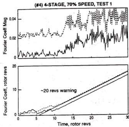
Fig. 1 Time history of first and second Fourier coefficients (Tryfonidis et al., 1995)
