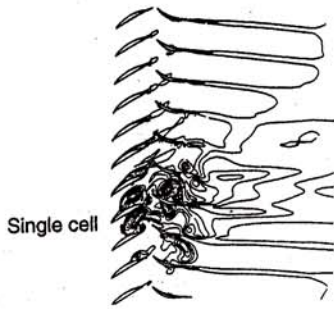
Fig. 5 Instantaneous entropy contour after stall inception from numerical simulation (He, 1997)
