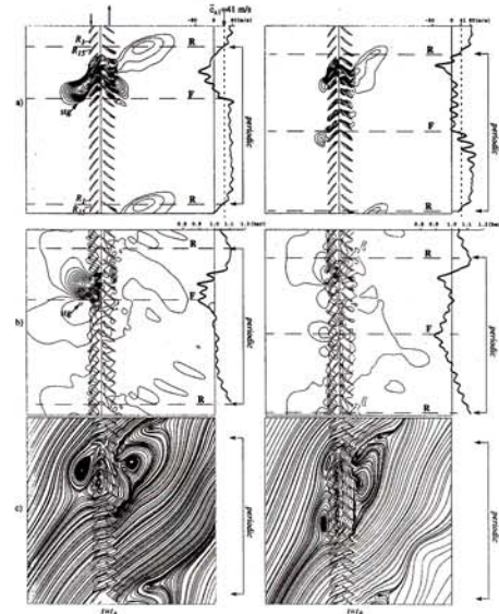
Fig. 6 (a) contours of negative axial velocity, (b) static pressure contours, (c) instantaneous cell-frame streamlines (Saxer-Felici et al, 1998)
