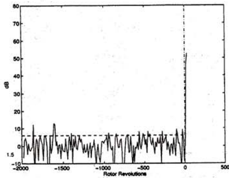
Fig. 4 Traveling wave energy in a NASA 35 rotor (Bright et al., 1997)
