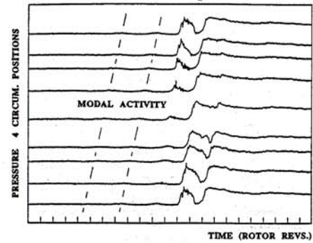
Fig. 2 Example of modes in a high-speed axial compressor (Day et al., 1999)
