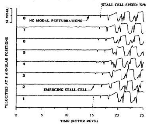
Fig. 3 Example of a spike type stall inception in an axial compressor. (Day, 1993)
