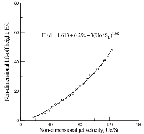
Fig. 6 Relation of non-dimensional lift-off height with non-dimensional jet velocity( V_o=0m/s )
