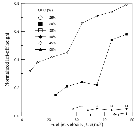
Fig. 8 Normalized lift-off heights for the flame using the general air( V_0=0.66 m/s)
