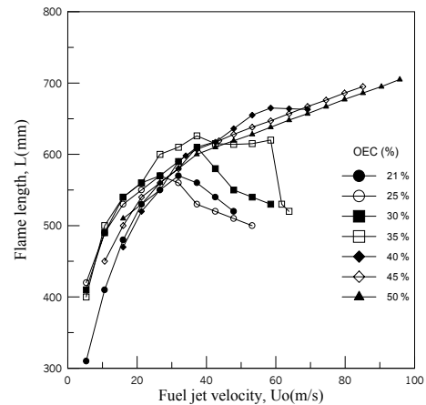
Fig. 9 Flame length with jet velocity for various OEC( V_0=0.66 m/s)
