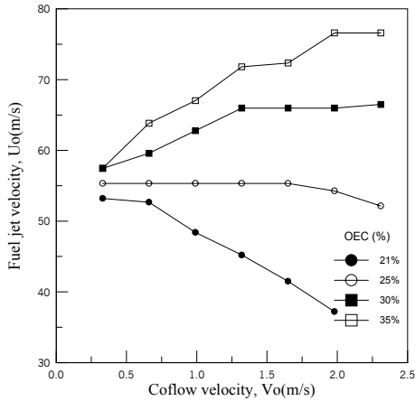
Fig. 4 Blowout limit with coflow velocity for various OECs
