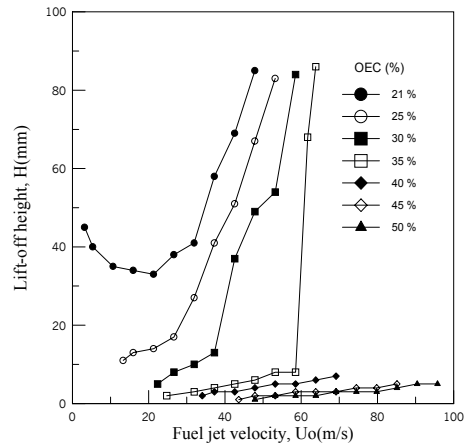
Fig. 7 Lift-off height with jet velocity for various OECs( V_o=0.66m/s )
