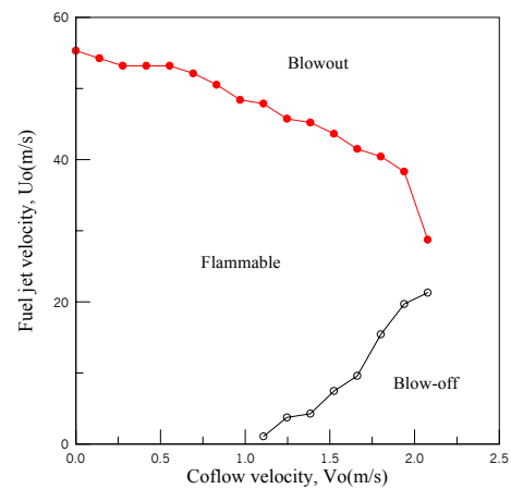
Fig. 3 Stability limit as a function of coflow velocity(OEC=21%)
