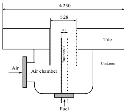
Fig. 2 Specification of the burner
