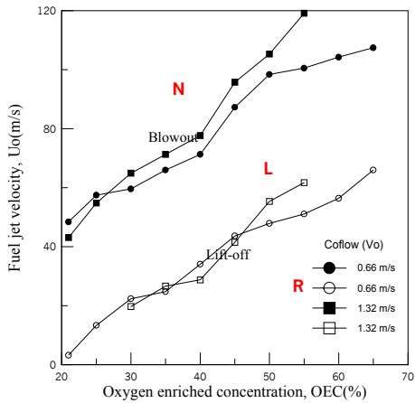
Fig. 5 Stability limit with OEC for two coflow velocity(N:no flame, L:lifted, R:rim attached)
