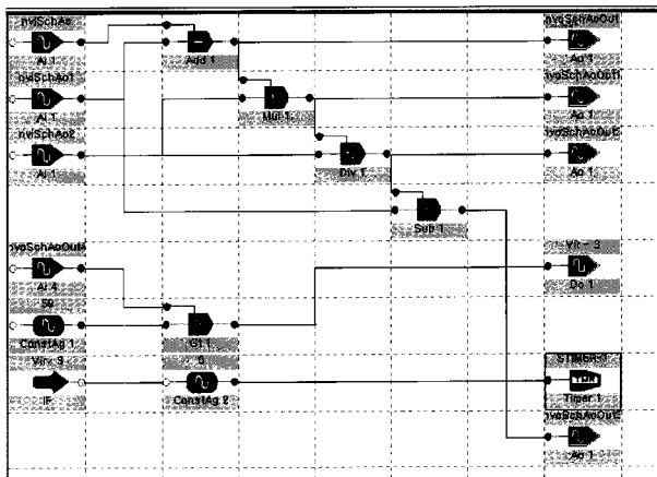
Fig. 6 Sequence of logic procedures
