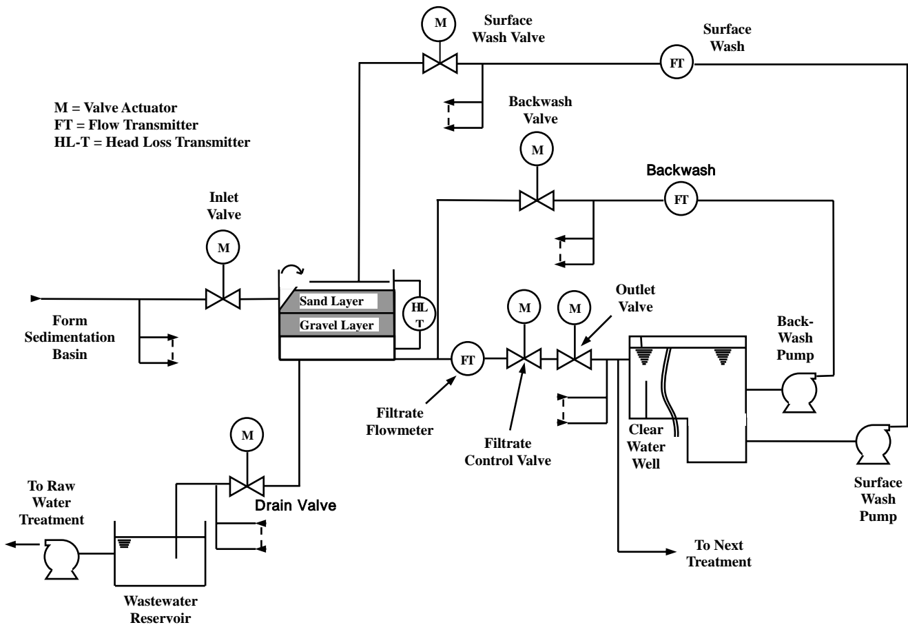
Fig. 2 Schematic of filter basin automation
