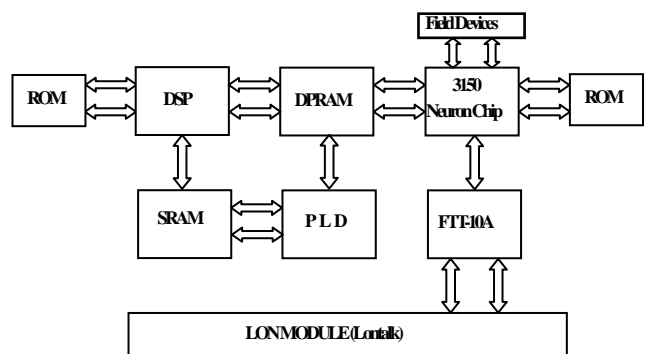
Fig. 3 Block diagram of master controller based on LonTalk protocol
