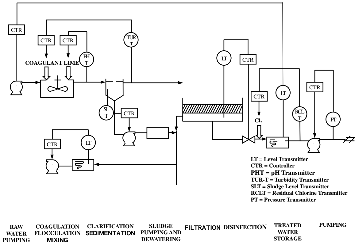
Fig.1. Schematic of a controlled treatment
