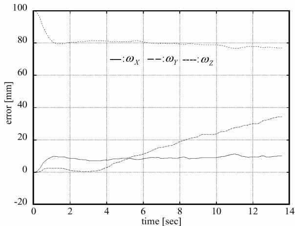
Fig. 6. Error in 3D for 3 Points (Vertical Stop).
