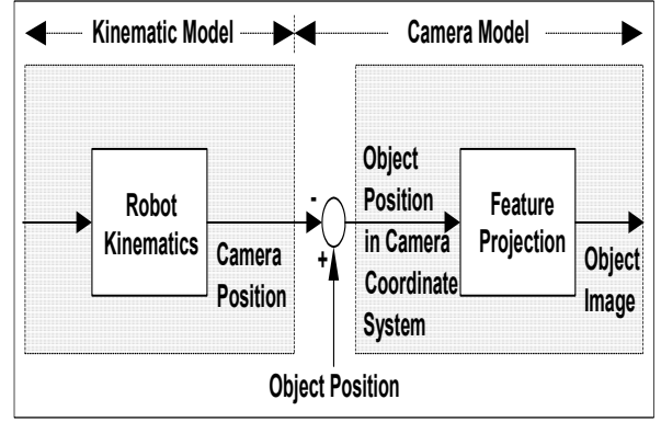
Fig. 1. System Modeling.
