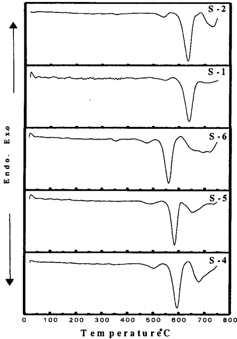
Fig. 2 DTA curve of BaO-ZnO-B 2 O 3 -V 2 O 5 glass(Transformation 450~500°C, Glass melting 550~590°C).
