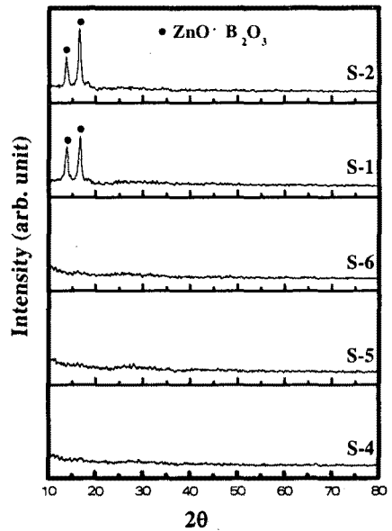
Fig. 1 XRD patterns of sample at 570℃.
