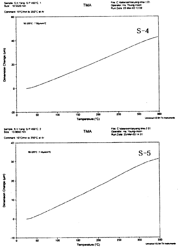
Fig. 4 Expansion coefficient of the S-4 and S-5.
