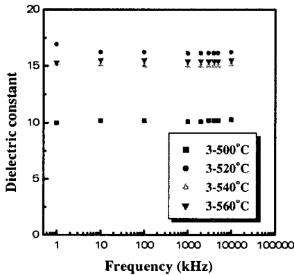
Fig. 3 Dielectric constance of heat treated sample.
