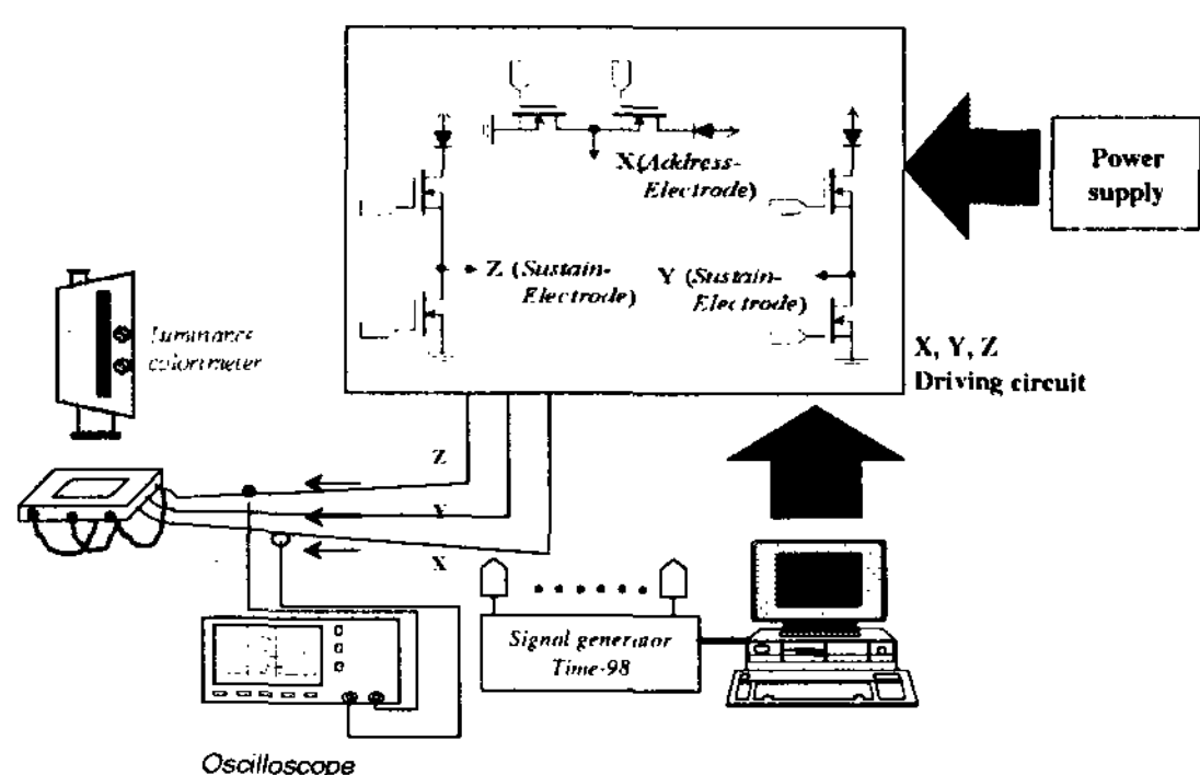
Figure 3. Schematic diagram of experimental setup
