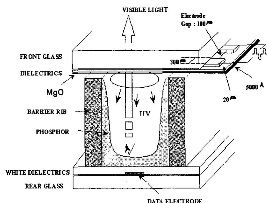
Figure 1. Principal structure of a discharge cell in ac PDP
