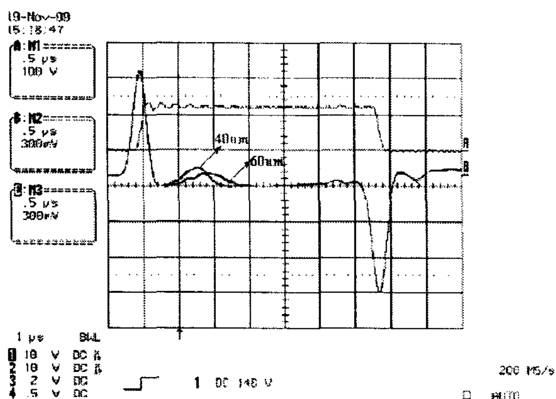
Figure 5. The current addressing discharge waveforms as a parameter of ITO gap
