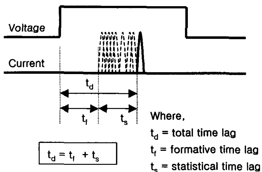
Figure 4. Discharge time lag
