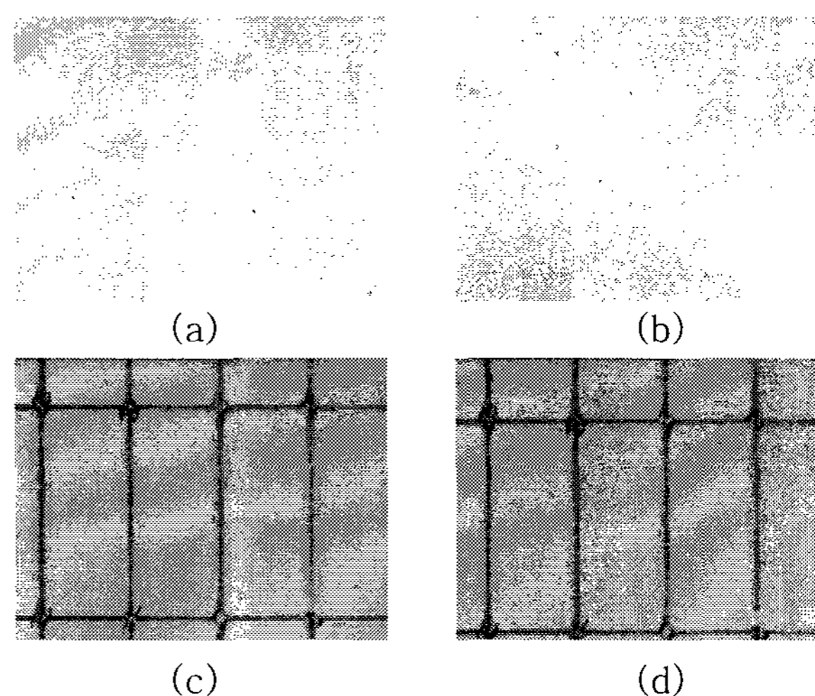
Fig. 5. Alignment textures before [(a) and (c)] and after [(b) and (d)] external pressure: (a) and (b) are normal SSFLC cell, and (c) and (d) are PIFLC cell.
