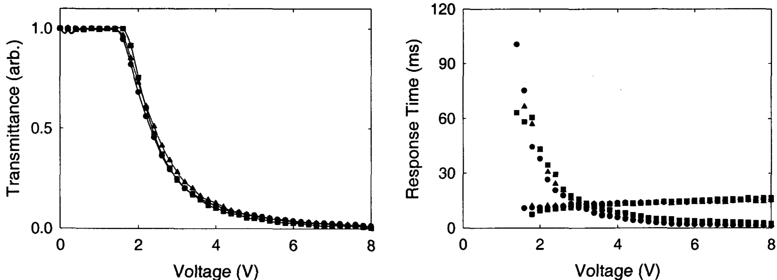
Fig. 6. Electro optical properties of normal (circle), PSCOF (triangle), and PINLC (square) as a function of applied voltages.
