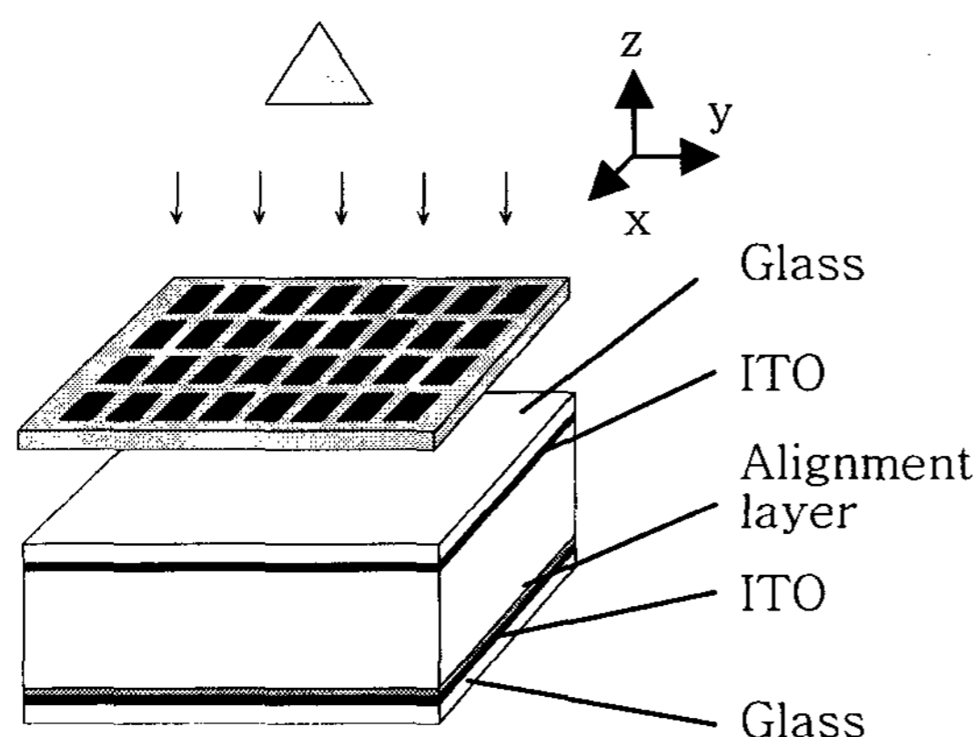
Fig. 1. Experimental set-up
