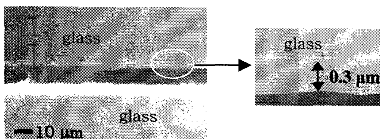
Fig.4. SEM image of PILC sample
