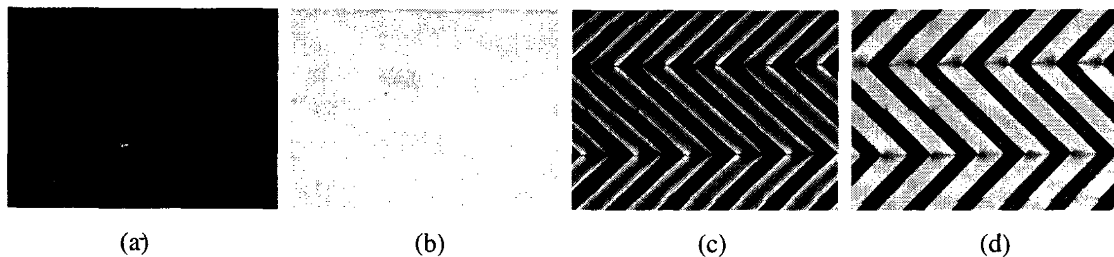
Fig. 1 Without applying field, (a) and (b) are the alignment textures when the rubbing direction is (a) parallel and (b) rotated 45^\circ with respect to the optic axis of analyzer. (c) and (d) are the textures with electric field of 0.5 \text{ V}/\mu\text{m} and 1 \text{ V}/\mu\text{m} , respectively. In (c) and (d), the rubbing direction is parallel to the analyzer.
