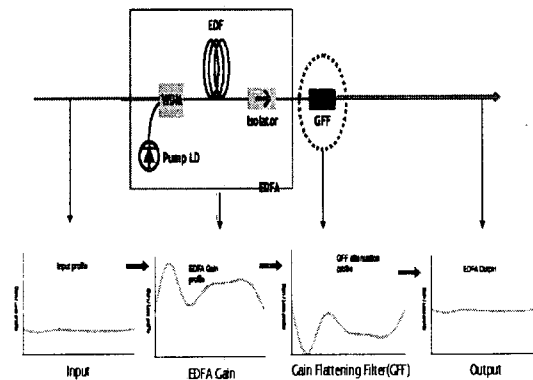
Figure 1. The effects of gain flattening filters
