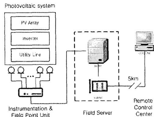
그림.1 Main Architecture of Monitoring system
