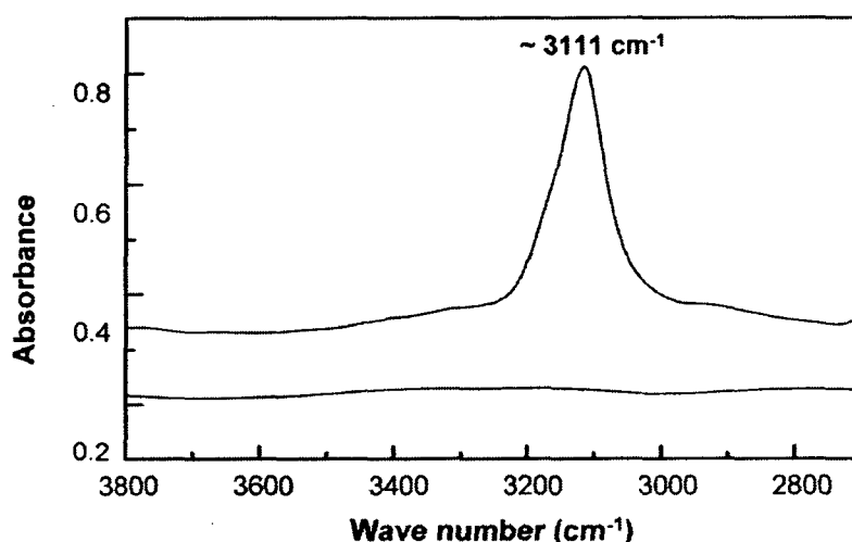
Figure 1. Polarized IR spectra of a single crystal of stishovite. The upper spectrum and the lower spectrum were obtained with incident IR light whose electric vector was perpendicular and parallel to the c axis, respectively.
