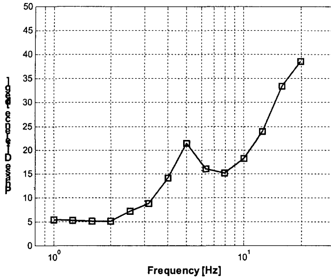
Figure 5. Phase difference between Korean and ISO apparent mass models.
