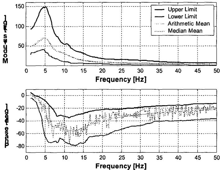
Figure 3. Characteristics of apparent mass under vertical vibration
