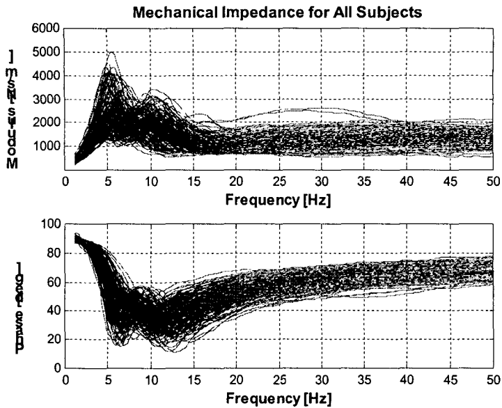
Figure 6. Total measurement set of Korean seated mechanical impedances under vertical vibration.
