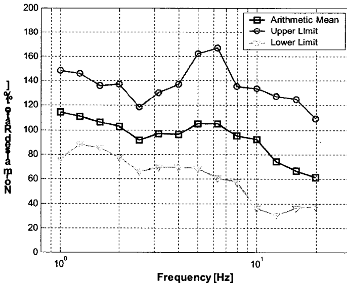
Figure 8. Normalised modulus ratio of Korean mechanical impedance to ISO/DIS 5982 model.
