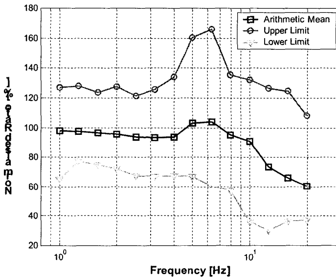
Figure 4. Normalised modulus ratio of measured Korean apparent mass to ISO 5982 model.
