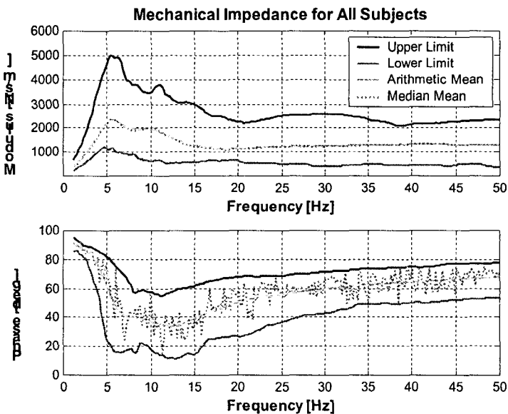
Figure 7. Characteristics of mechanical impedance under vertical vibration.
