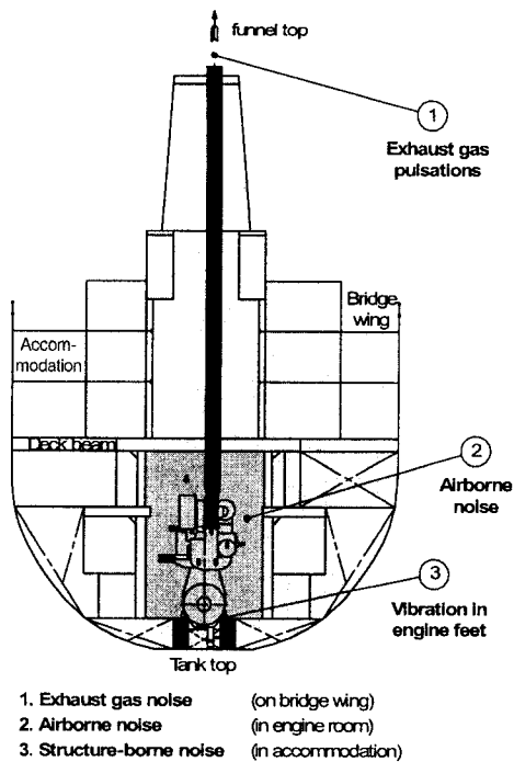
Fig. 4: Typical sources of engine noise
