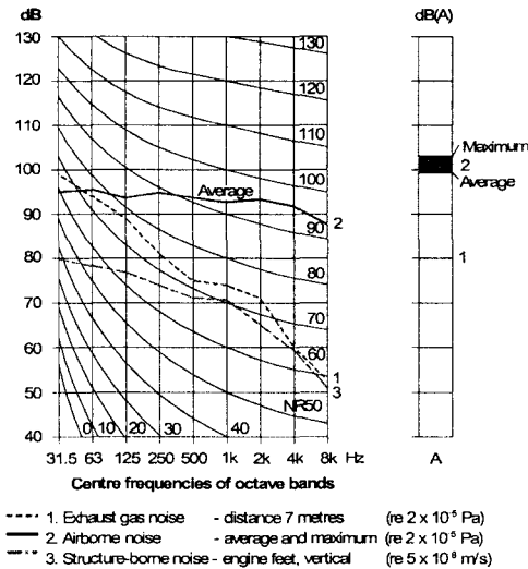
Fig. 7b: ISO's NR curves and noise levels for a 6S26MC Mk 6 engine. MCR: 2,400 kW at 250 r/min.
