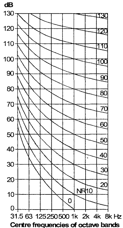
Fig. 2: ISO's Noise Rating curves Octave band pressure levels, re 2 \times 10^{-5} \text{ Pa}
