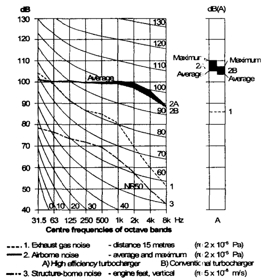
Fig. 7a: ISO's NR curves and noise levels for a 6L80MC Mk 5 engine. MCR: 20,580 kW at 93 r/m.n.
