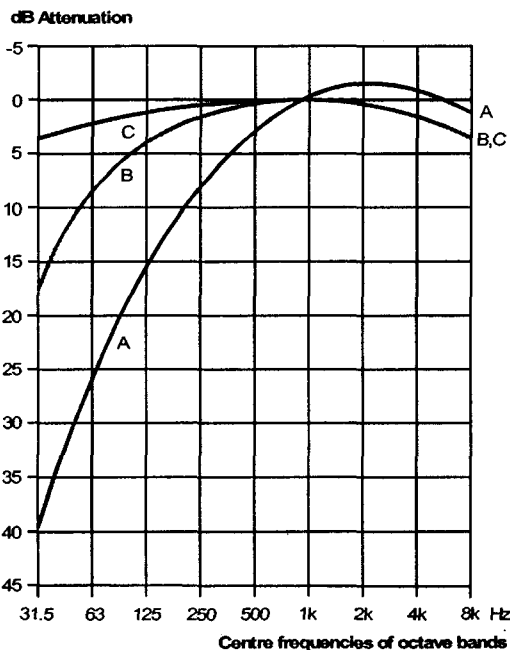
Fig. 3: Filtering (weighting) curves for sound level meters
