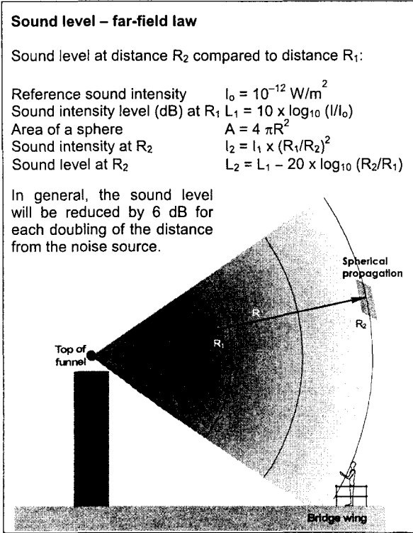
Fig. 1: Spherically propagated sound waves – far-field law. Distance R from noise source (point source assumed)
