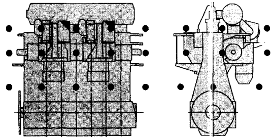
Fig. 6: Example of location of measuring points on a diesel engine in accordance with CIMAC's recommendations of measurement
