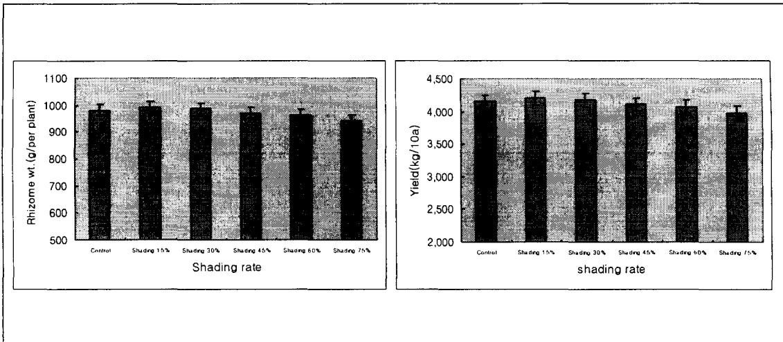
Fig.2. Comparison of different Shading on the rhizome weight of Curcuma aromatica Salisbury
