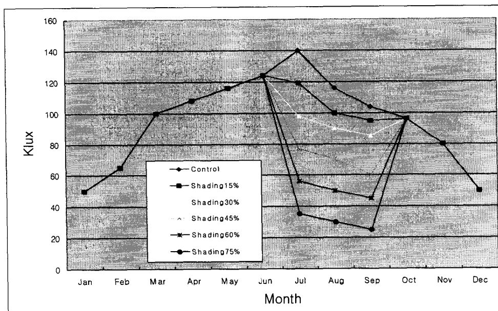
Fig. 1. Monthly changes of light intensity at Imhoemyeon in Jindo, Korea
