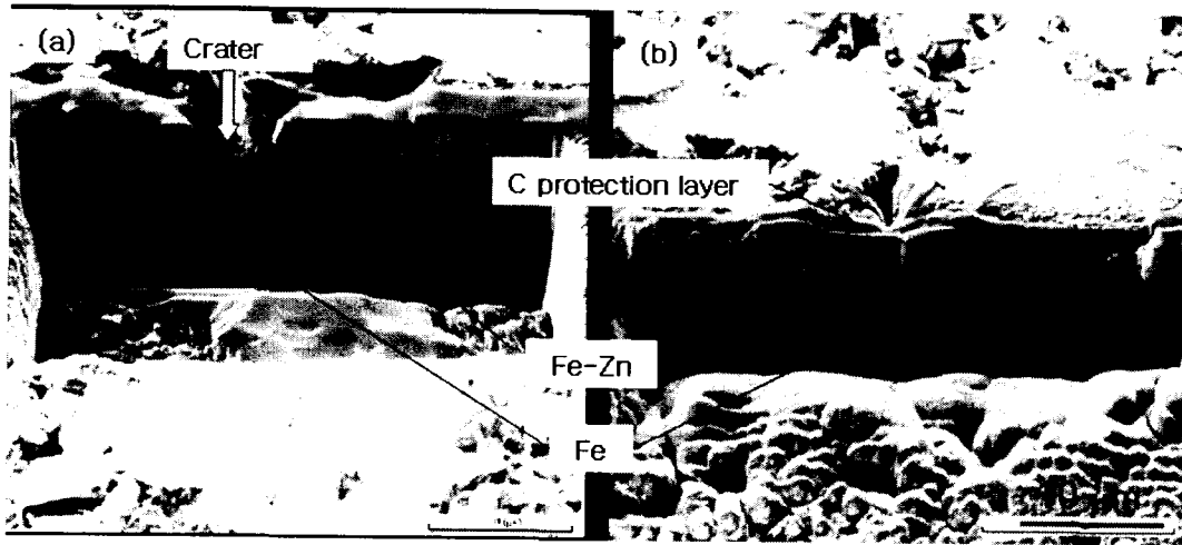
Figure 1. FIB images obtained from (a) normal and (b) defected GA coating
