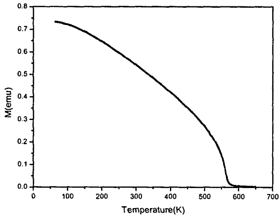
Fig. 2. Temperature dependence of magnetic moment under an applied of 5 kOe for Y_{2.9}Ce_{0.1}Fe_5O_{12} powder.
