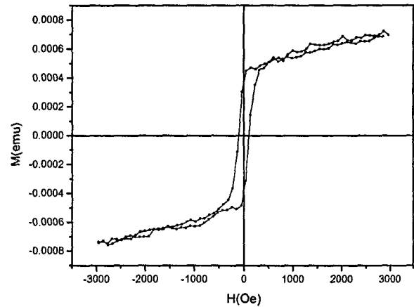
Fig. 3. M-H Curves of La_{0.67}Sr_{0.33}MnO_3/SiO_2/Si thin film at room temperature.
