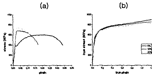
Fig. 4 Stress-strain curves of Low-Si steel with the variation of the strain amount of drawing in (a) tensile test, (b) compression test
