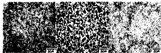
Fig. 2 Optical Micrographs for steels (Nital etching) (a) DP steel (b) Low-Si steel (c) ULCB steel
