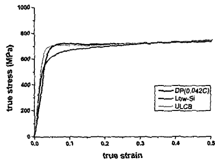
Fig. 6 Compressive stress-strain curves of three different steels after 20% drawing
