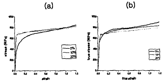
Fig. 5 Compressive stress-strain curves of with the variation of the strain amount of drawing. (a) DP steel, (b) ULCB steel
