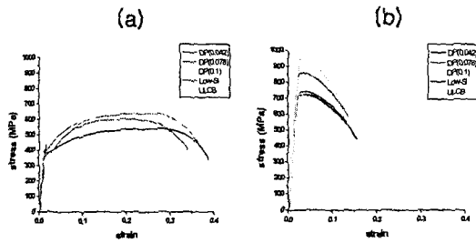
Fig. 3 Tensile stress-strain curves of three different steels (a) without drawing, (b) with drawing ( \epsilon = 0.2 )
