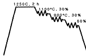
Fig. 1 The diagram for hot rolling conditions
