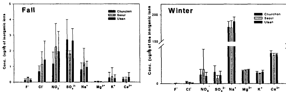
Fig. 1. Comparison of the concentrations ( \mu\text{g}/\text{m}^3 ) of inorganic ions in \text{PM}_{2.5} collected from three cities in the fall and winter of 2002-2003.
