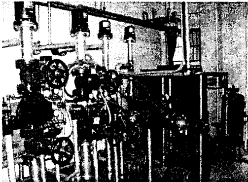
Fig. 2. Sprinkler systems
