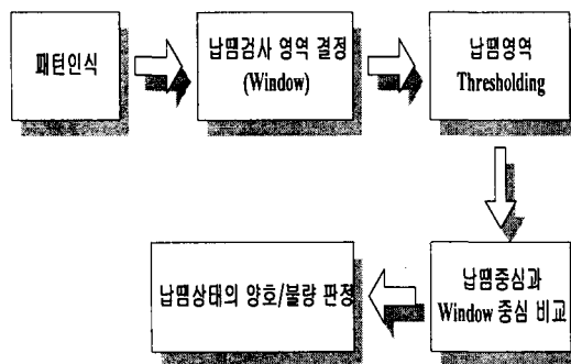
Fig. 1 Flowchart of solder test.
