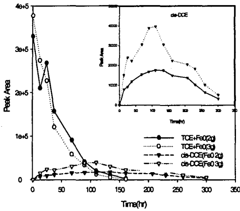
Fig. 1. Degradation of 100ppm TCE by zero-valent iron
